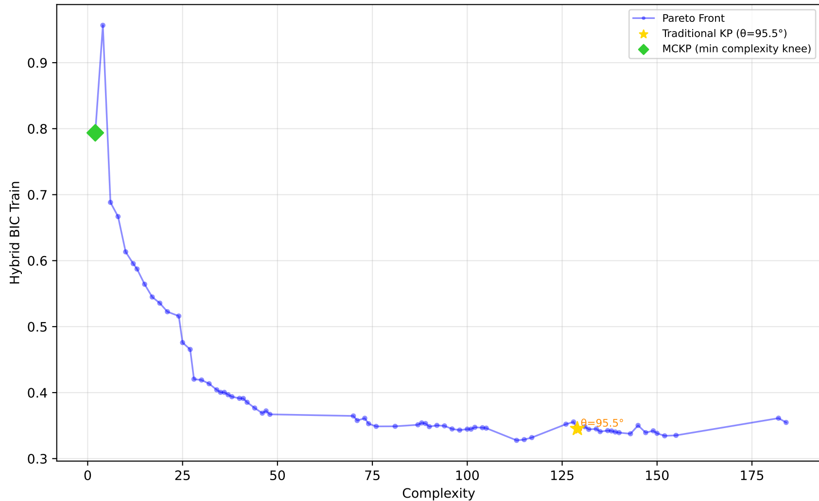
561_cpu - Run 29 - MVP - Hybrid BIC Train \lambda_1=0.50, \lambda_2=0.20, \lambda_3=0.00 | Difficulty: 1.00 | Method: hmr
