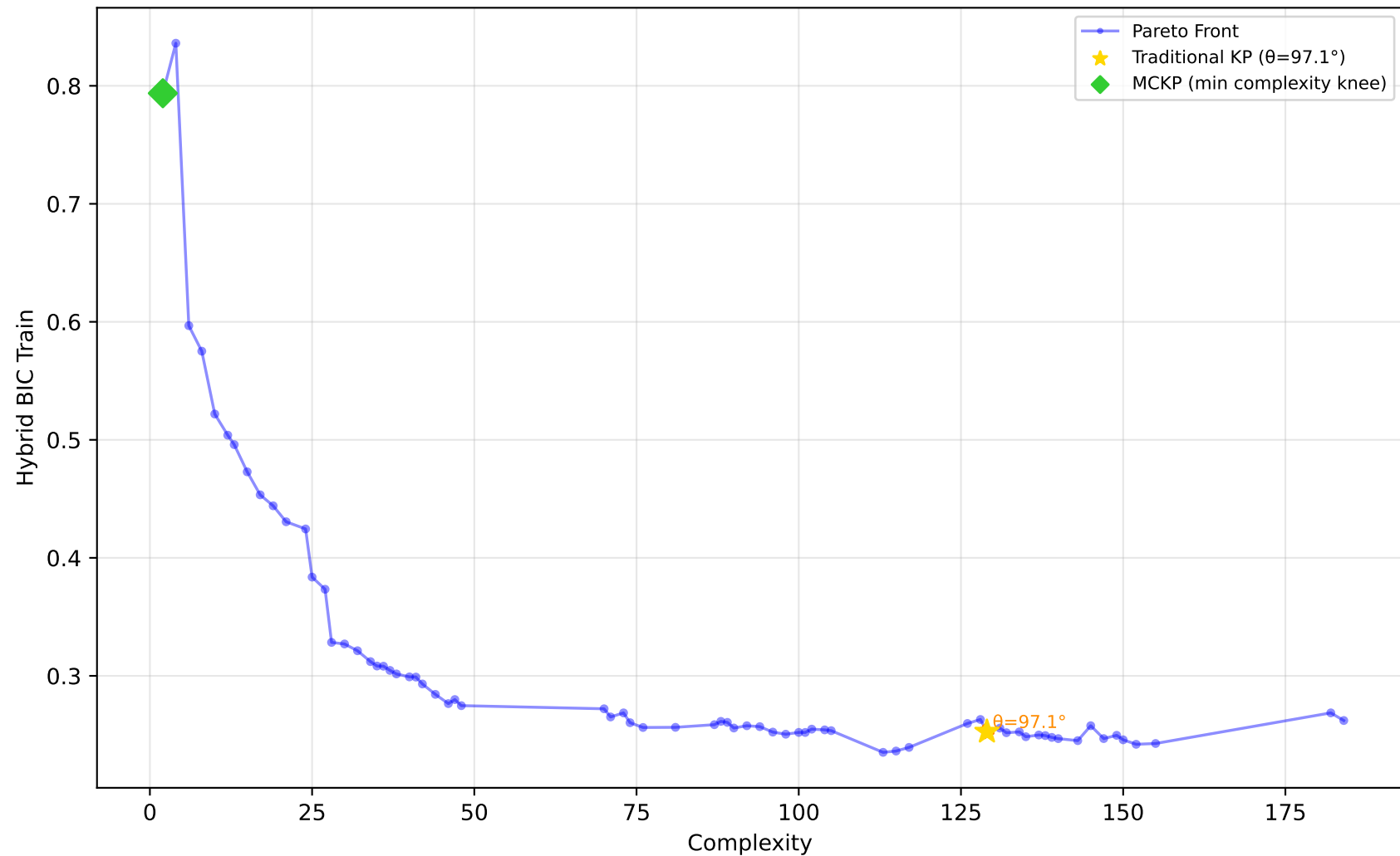
561_cpu - Run 29 - MVP - Hybrid BIC Train \lambda_1=0.70, \lambda_2=0.00, \lambda_3=0.10 | Difficulty: 1.00 | Method: hmr
