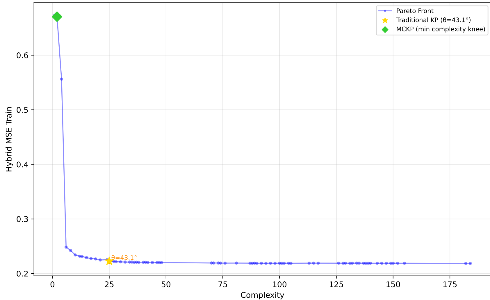
561_cpu - Run 29 - MVP - Hybrid MSE Train \lambda_1=0.50, \lambda_2=0.20, \lambda_3=0.00 | Difficulty: 1.00 | Method: hmr
