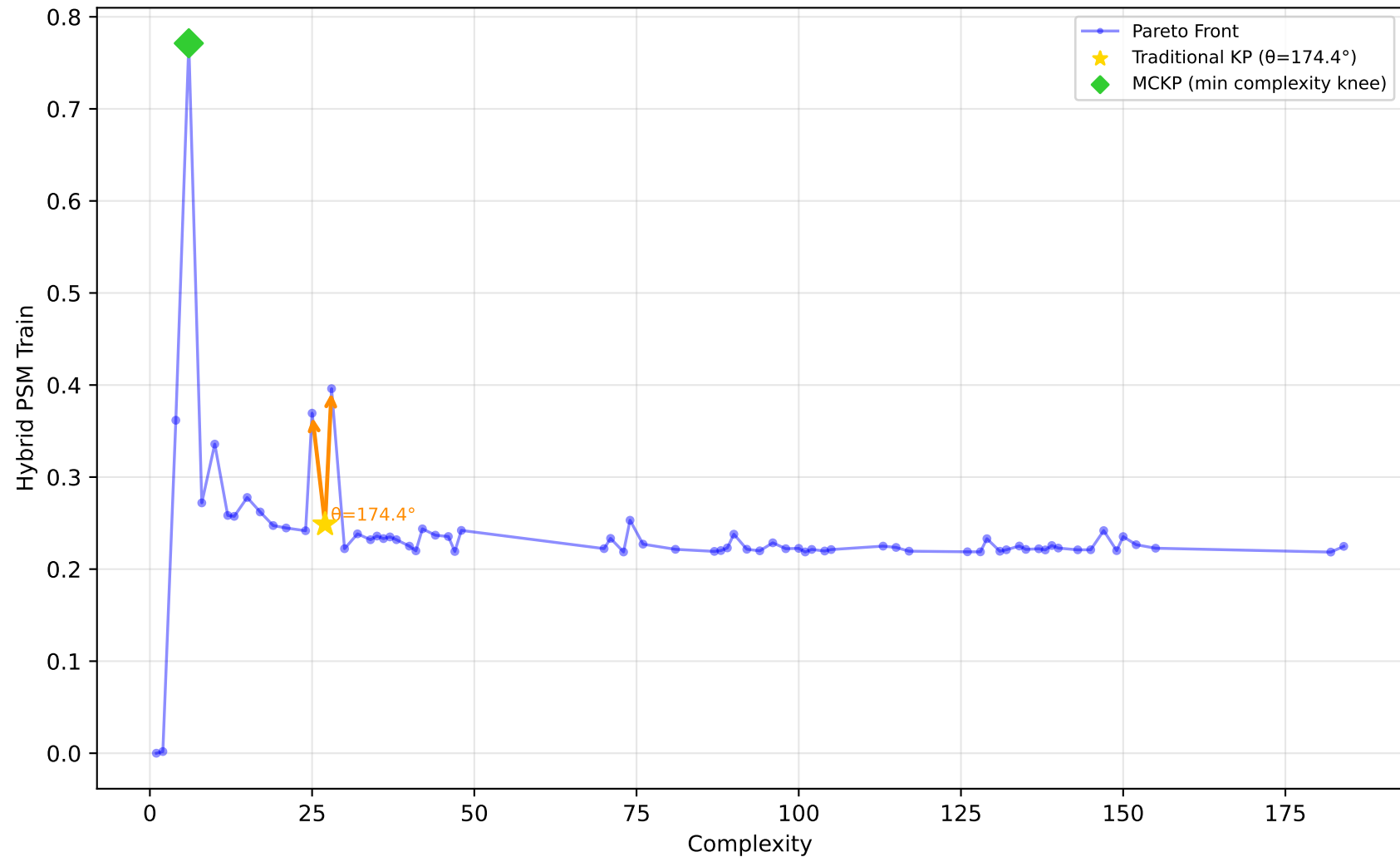
561_cpu - Run 29 - MVP - Hybrid PSM Train \lambda_1=0.50, \lambda_2=0.20, \lambda_3=0.00 | Difficulty: 1.00 | Method: hmr
