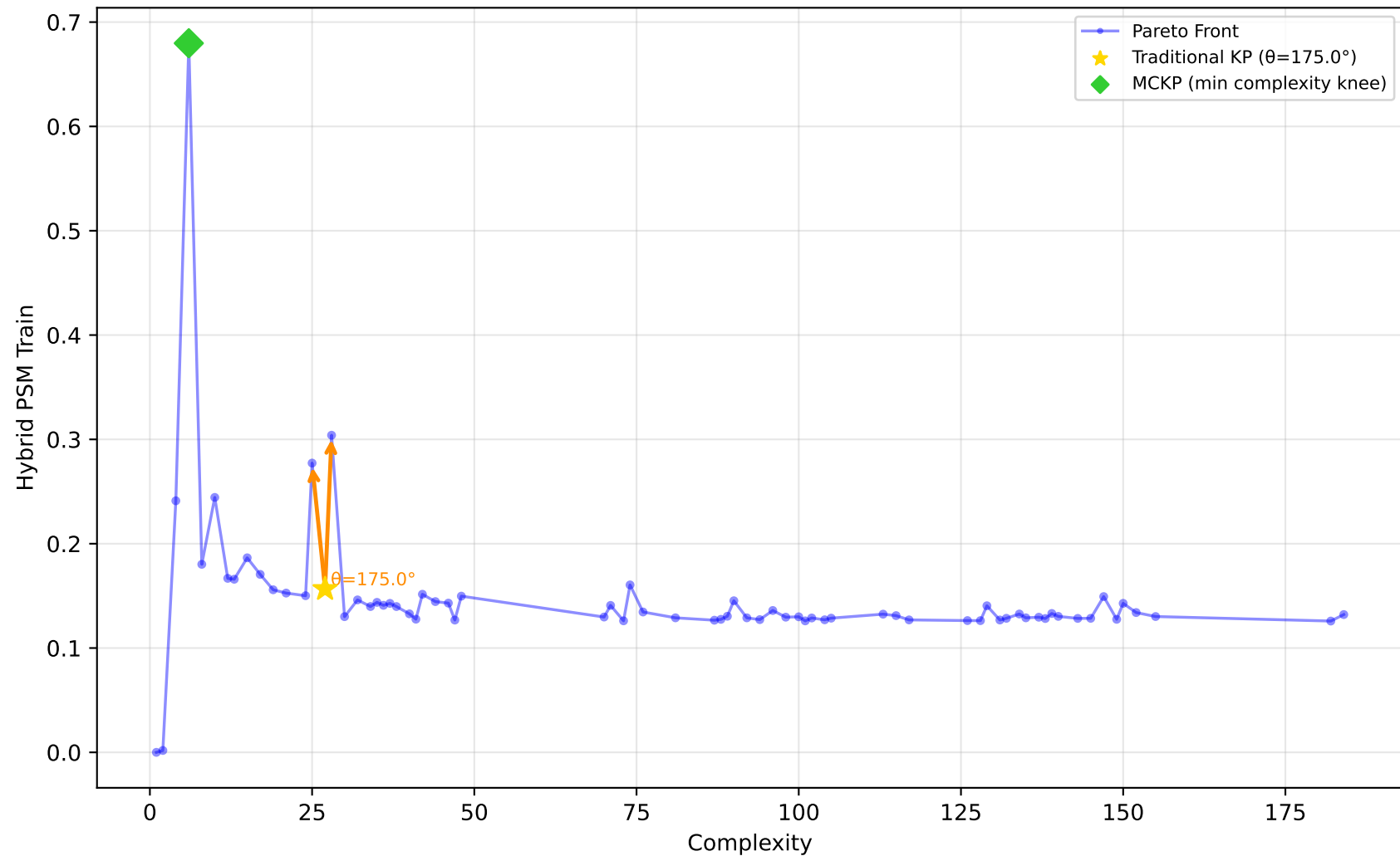
561_cpu - Run 29 - MVP - Hybrid PSM Train \lambda_1=0.70, \lambda_2=0.00, \lambda_3=0.10 | Difficulty: 1.00 | Method: hmr
