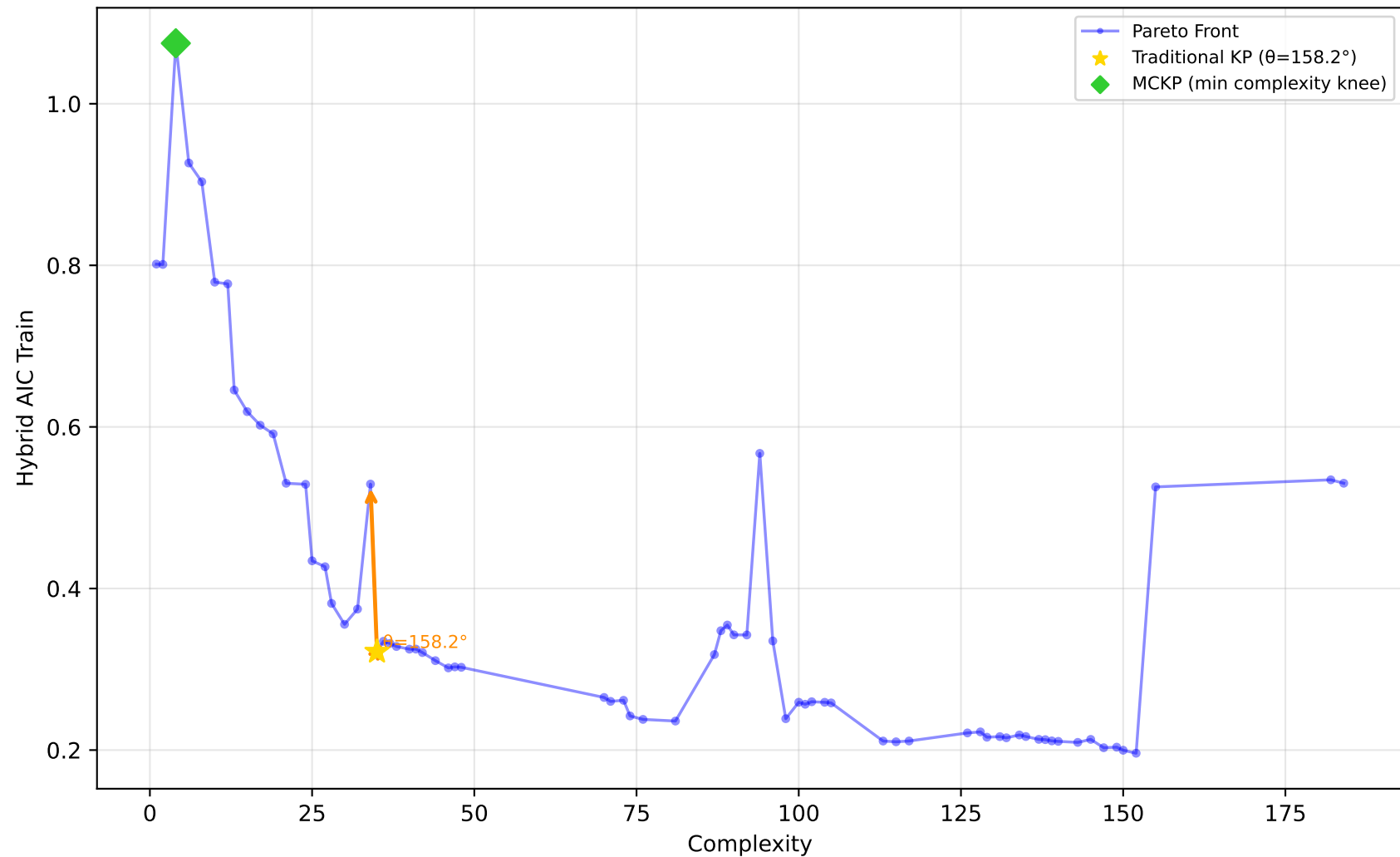
561_cpu - Run 29 - SVP - Hybrid AIC Train \lambda_1=1.00, \lambda_2=0.00, \lambda_3=0.40 | Difficulty: 1.00 | Method: hmr
