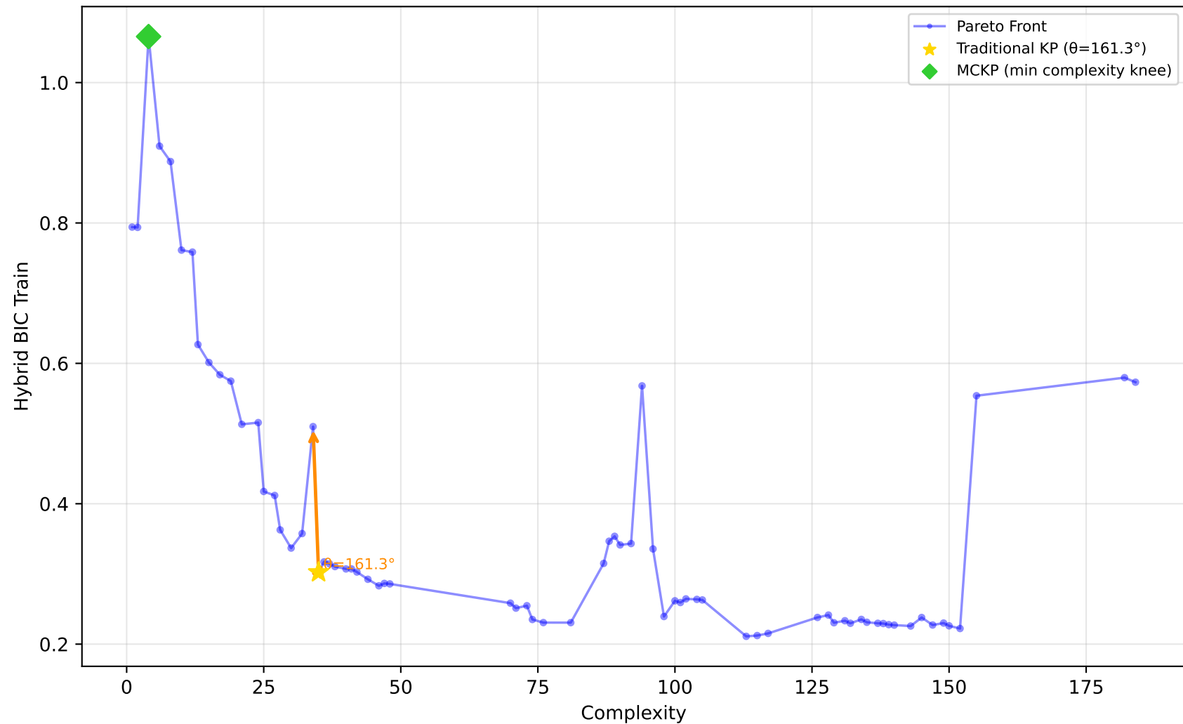
561_cpu - Run 29 - SVP - Hybrid BIC Train \lambda_1=1.00, \lambda_2=0.00, \lambda_3=0.40 | Difficulty: 1.00 | Method: hmr
