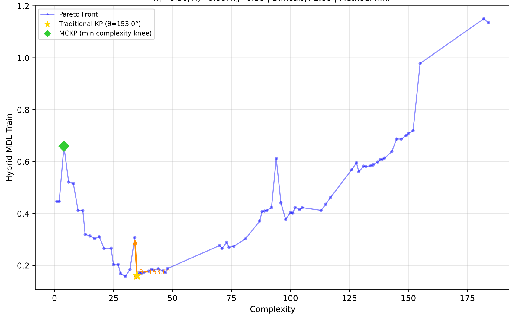
561_cpu - Run 29 - SVP - Hybrid MDL Train \lambda_1=0.90, \lambda_2=0.00, \lambda_3=0.30 | Difficulty: 1.00 | Method: hmr
