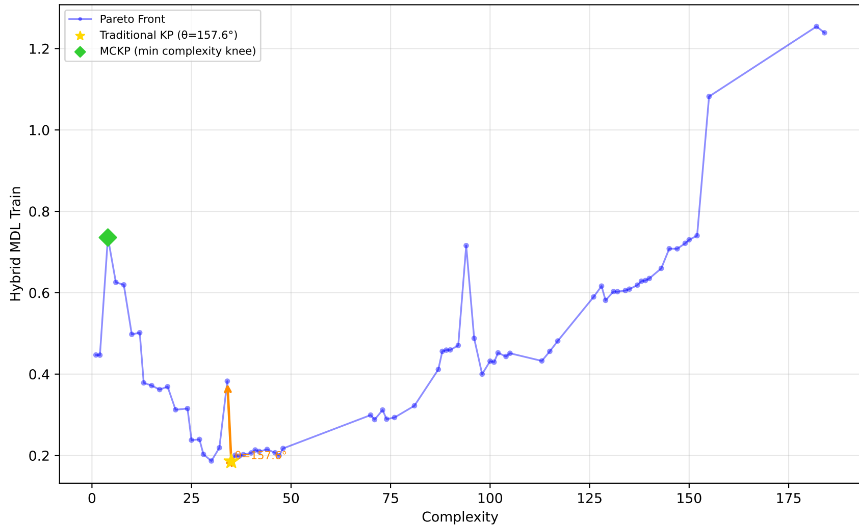
561_cpu - Run 29 - SVP - Hybrid MDL Train \lambda_1=1.00, \lambda_2=0.00, \lambda_3=0.40 | Difficulty: 1.00 | Method: hmr
