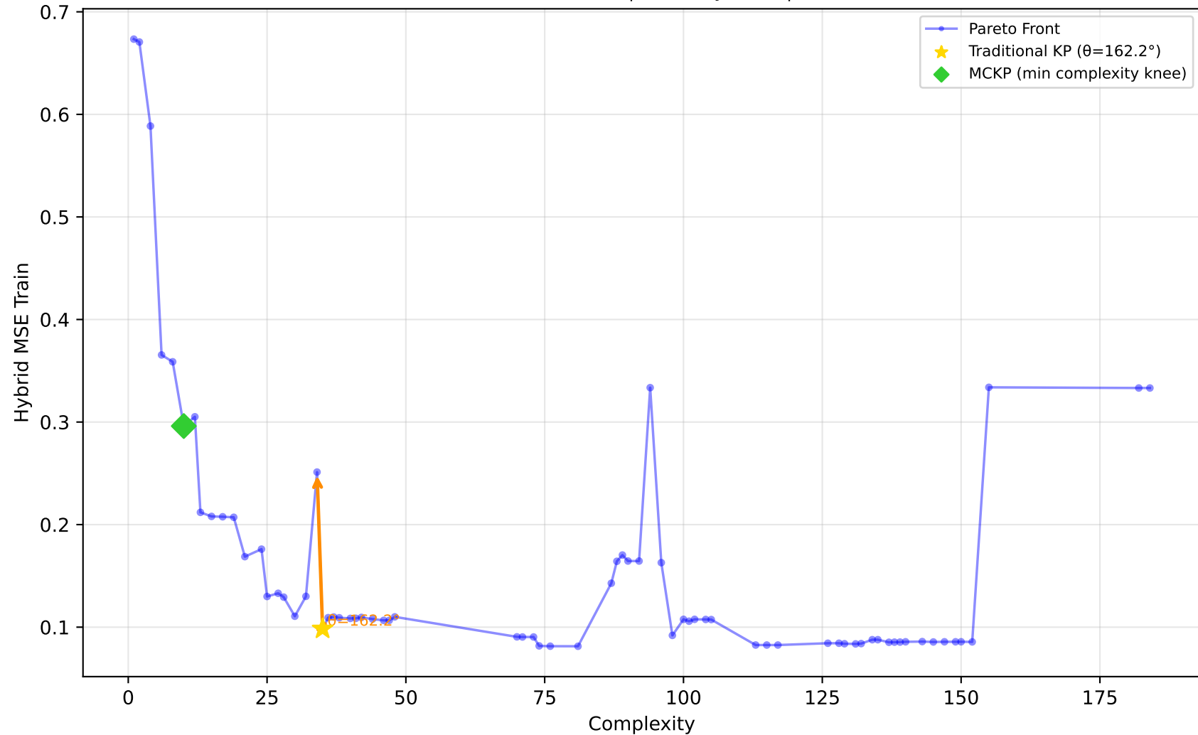
561_cpu - Run 29 - SVP - Hybrid MSE Train \lambda_1=0.90, \lambda_2=0.00, \lambda_3=0.30 | Difficulty: 1.00 | Method: hmr
