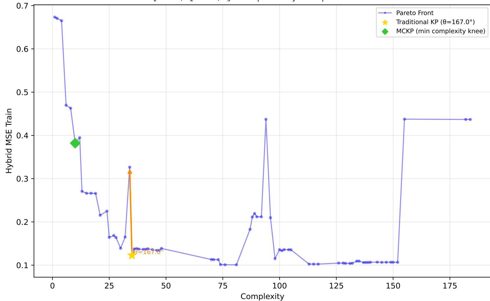
561_cpu - Run 29 - SVP - Hybrid MSE Train \lambda_1=1.00, \lambda_2=0.00, \lambda_3=0.40 | Difficulty: 1.00 | Method: hmr
