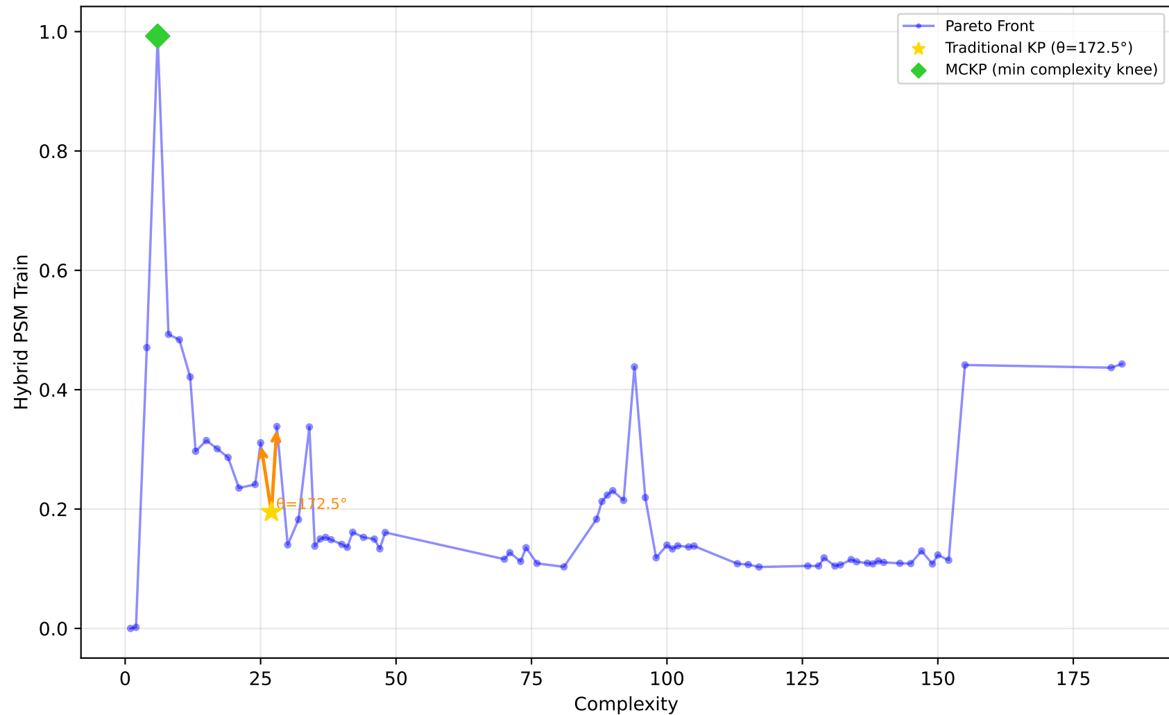
561_cpu - Run 29 - SVP - Hybrid PSM Train \lambda_1=1.00, \lambda_2=0.00, \lambda_3=0.40 | Difficulty: 1.00 | Method: hmr
