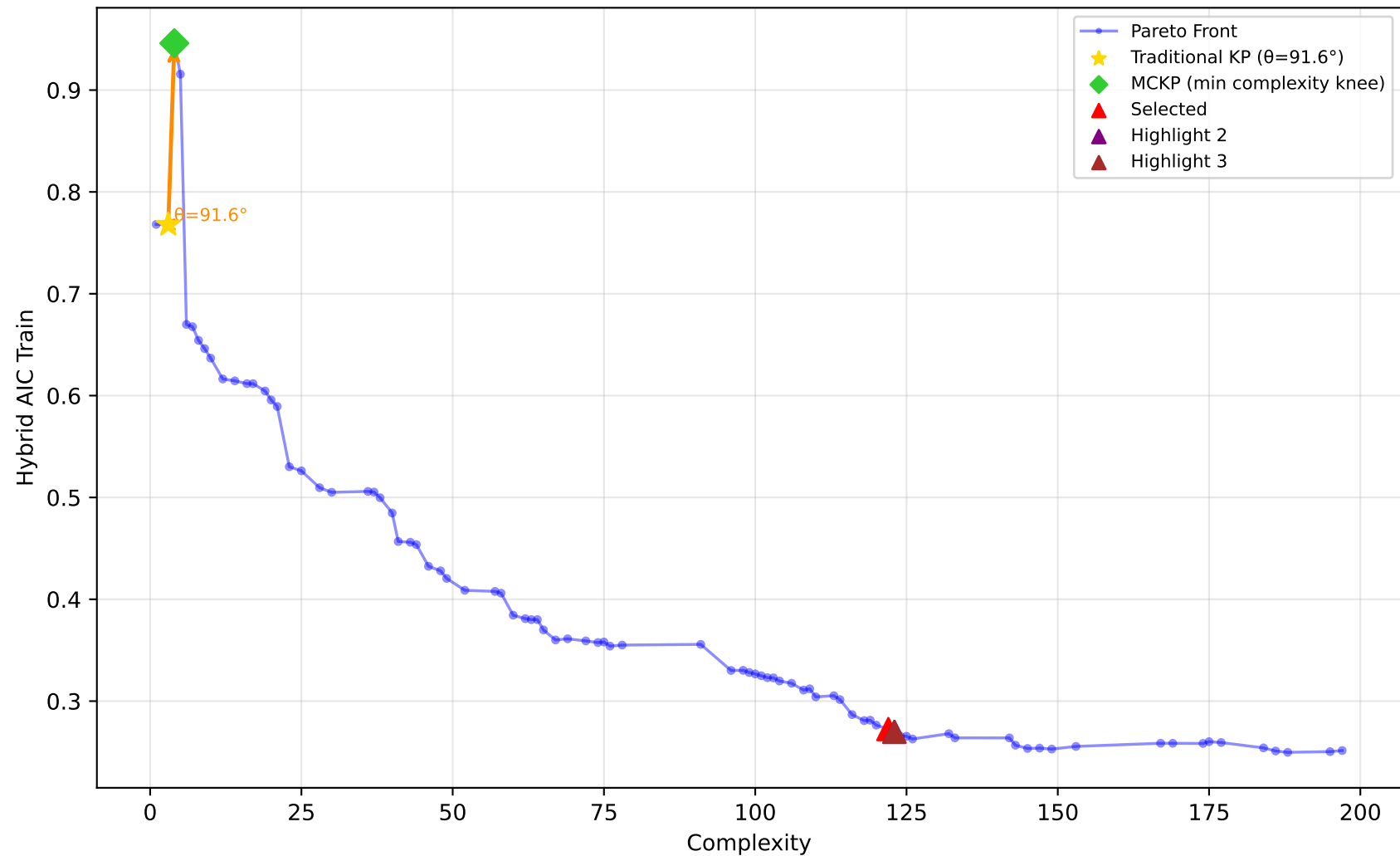
561_cpu - Run 2 - MVP - Hybrid AIC Train \lambda_1=0.70, \lambda_2=0.00, \lambda_3=0.10 | Difficulty: 0.51 | Method: mckp
