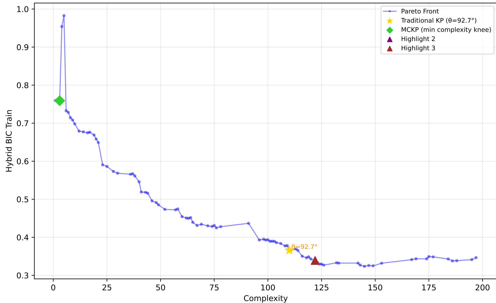
561_cpu - Run 2 - MVP - Hybrid BIC Train \lambda_1=0.50, \lambda_2=0.20, \lambda_3=0.00 | Difficulty: 0.51 | Method: mckp
