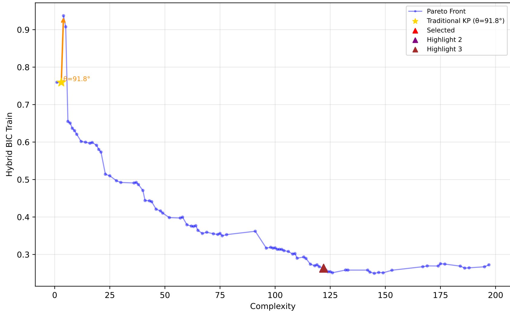
561_cpu - Run 2 - MVP - Hybrid BIC Train \lambda_1=0.70, \lambda_2=0.00, \lambda_3=0.10 | Difficulty: 0.51 | Method: mckp
