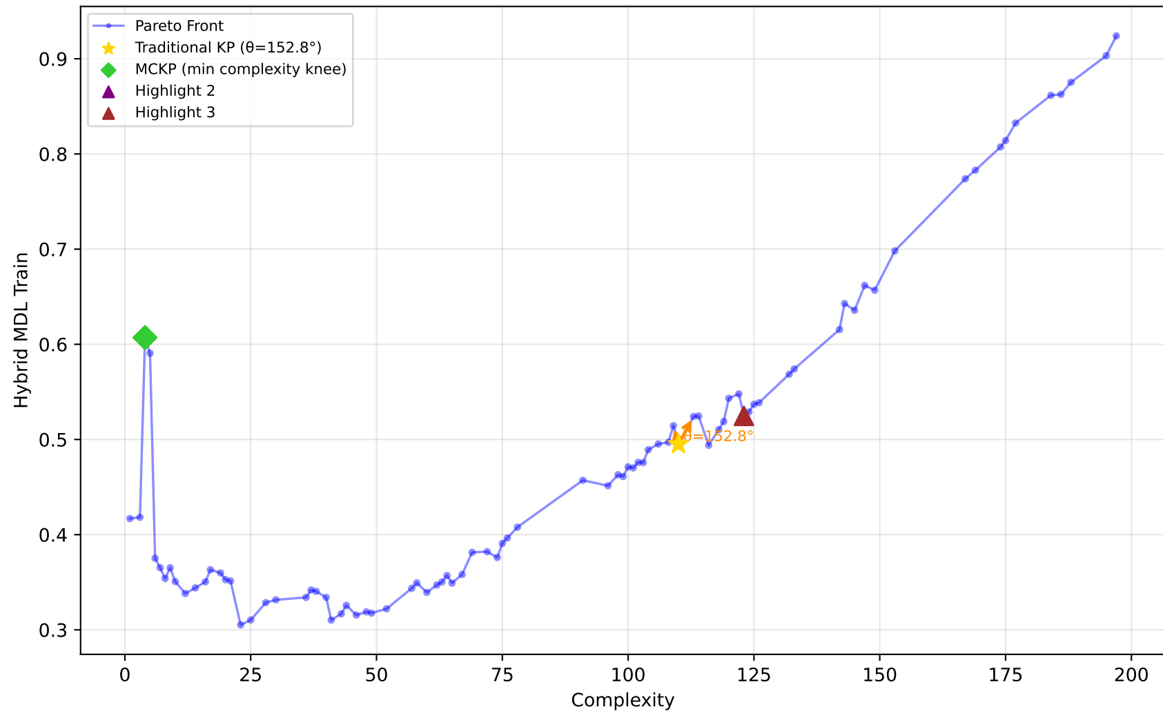
561_cpu - Run 2 - MVP - Hybrid MDL Train \lambda_1=0.70, \lambda_2=0.00, \lambda_3=0.10 | Difficulty: 0.51 | Method: mckp
