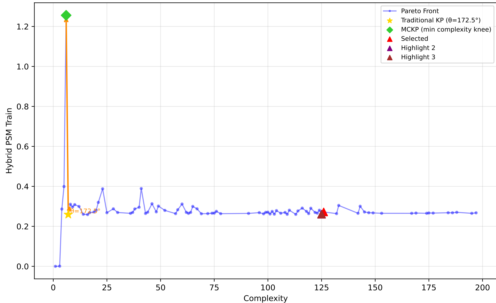
561_cpu - Run 2 - MVP - Hybrid PSM Train \lambda_1=0.50, \lambda_2=0.20, \lambda_3=0.00 | Difficulty: 0.51 | Method: mckp
