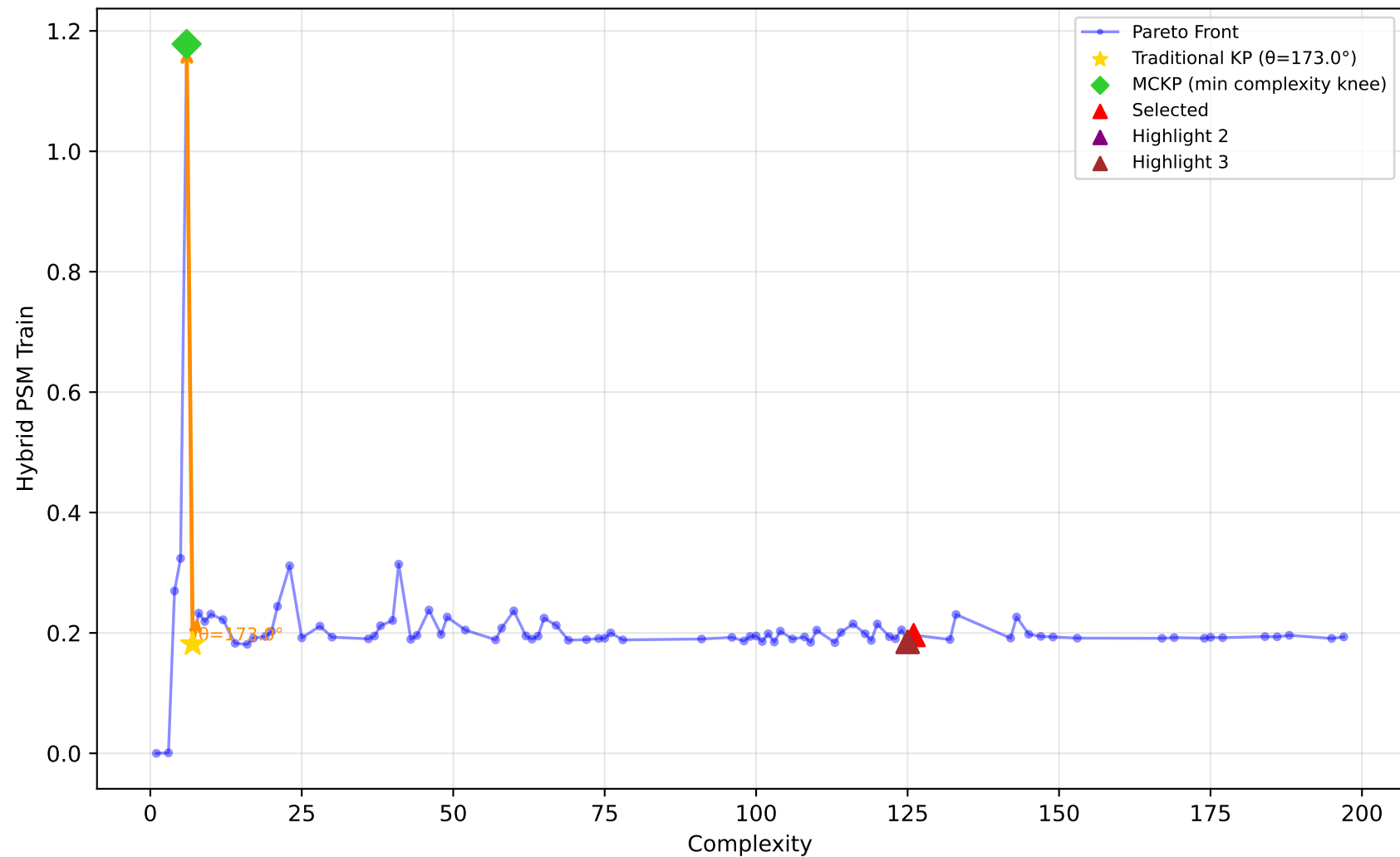
561_cpu - Run 2 - MVP - Hybrid PSM Train \lambda_1=0.70, \lambda_2=0.00, \lambda_3=0.10 | Difficulty: 0.51 | Method: mckp
