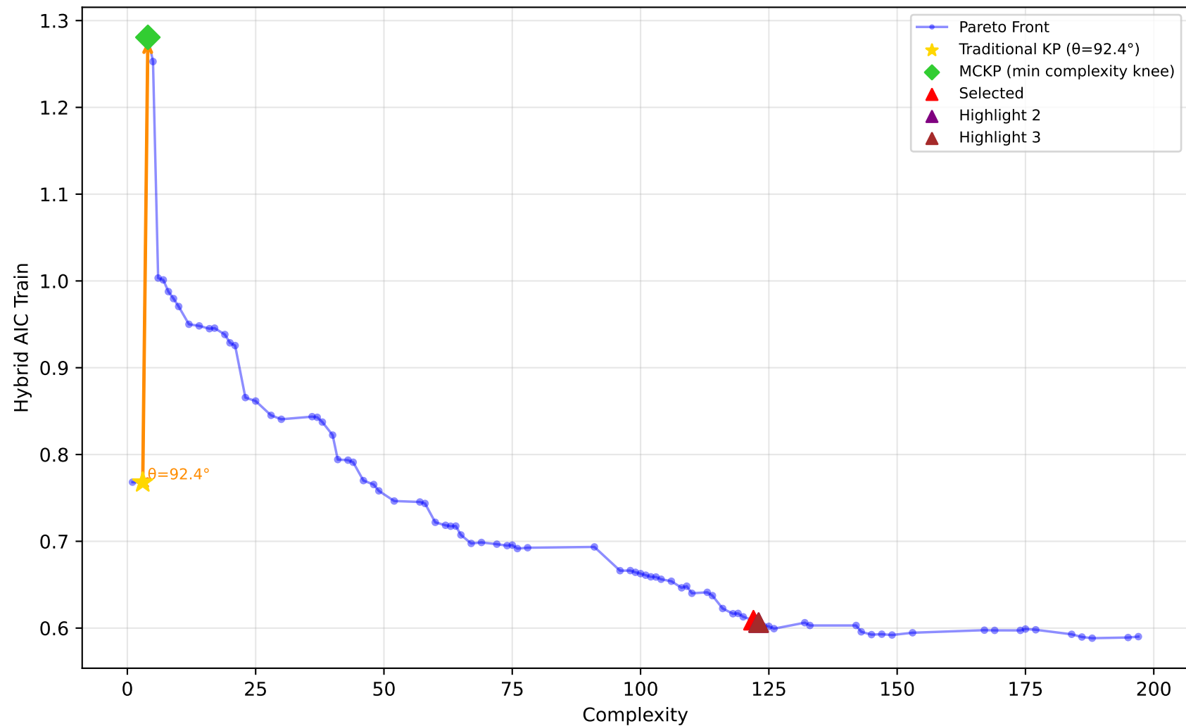
561_cpu - Run 2 - SVP - Hybrid AIC Train \lambda_1=1.00 , \lambda_2=0.00 , \lambda_3=0.40 | Difficulty: 0.51 | Method: mckp
