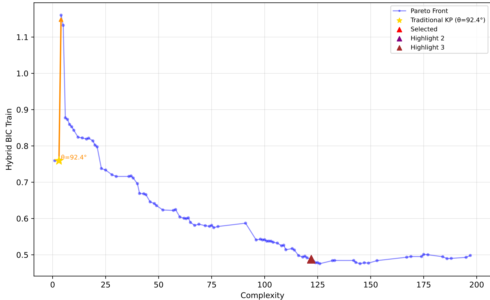
561_cpu - Run 2 - SVP - Hybrid BIC Train \lambda_1=0.90, \lambda_2=0.00, \lambda_3=0.30 | Difficulty: 0.51 | Method: mckp
