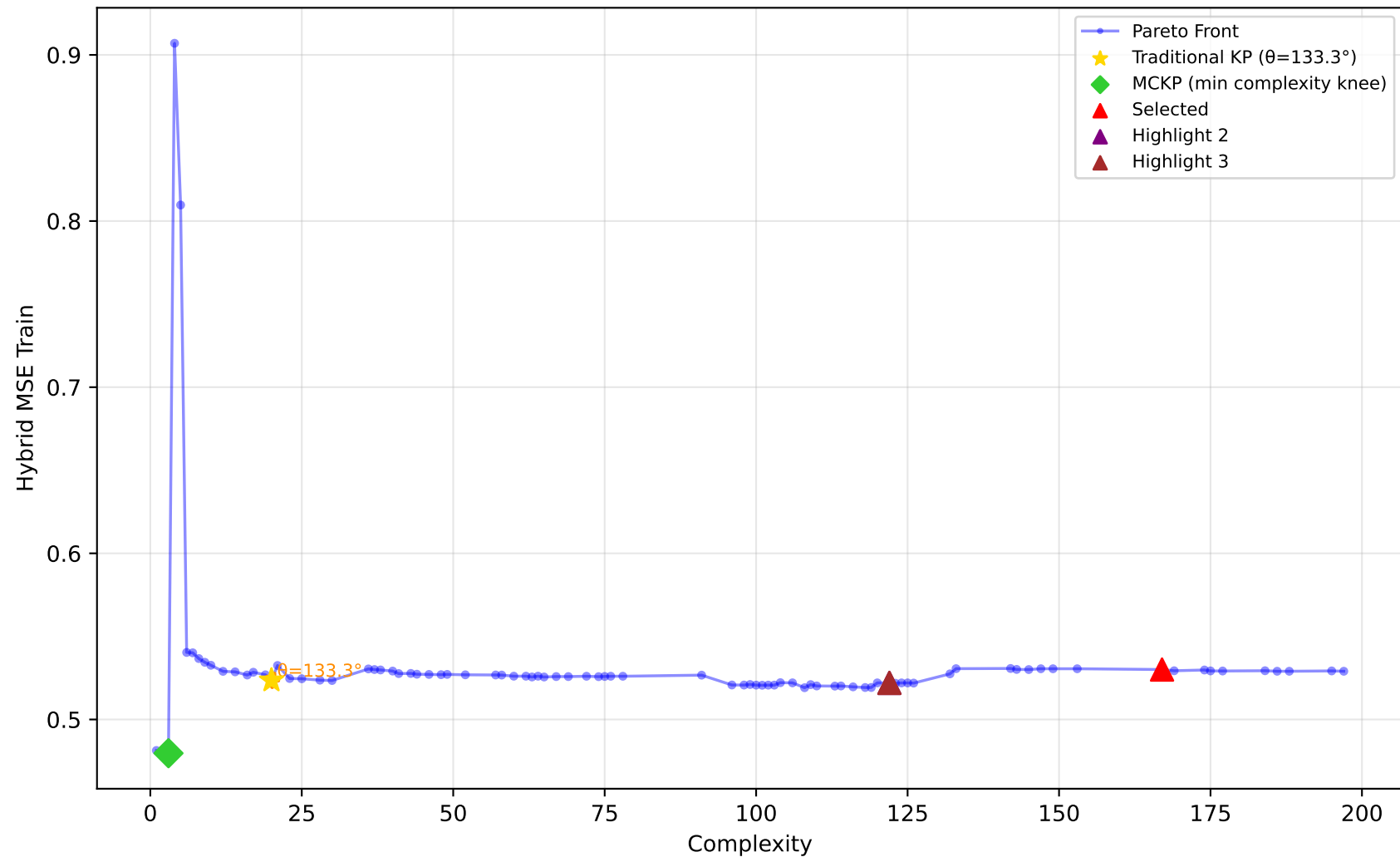
561_cpu - Run 2 - SVP - Hybrid MSE Train \lambda_1=1.00, \lambda_2=0.00, \lambda_3=0.40 | Difficulty: 0.51 | Method: mckp
