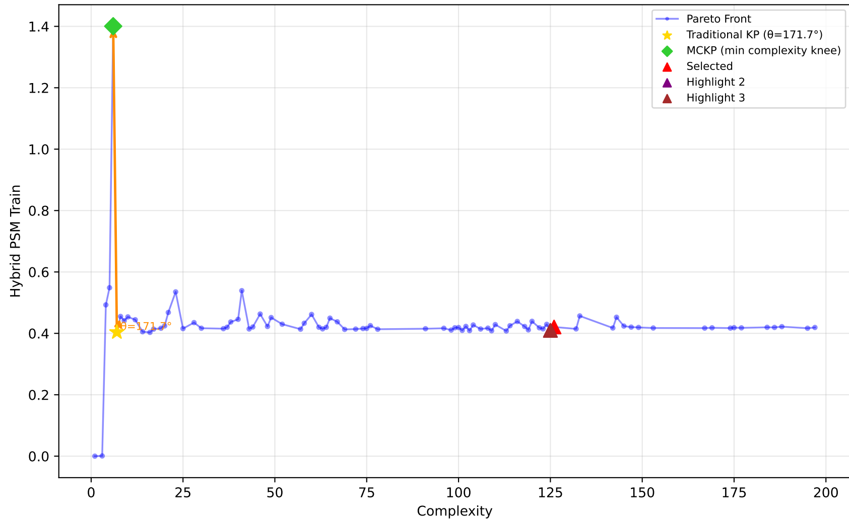
561_cpu - Run 2 - SVP - Hybrid PSM Train \lambda_1=0.90, \lambda_2=0.00, \lambda_3=0.30 | Difficulty: 0.51 | Method: mckp
