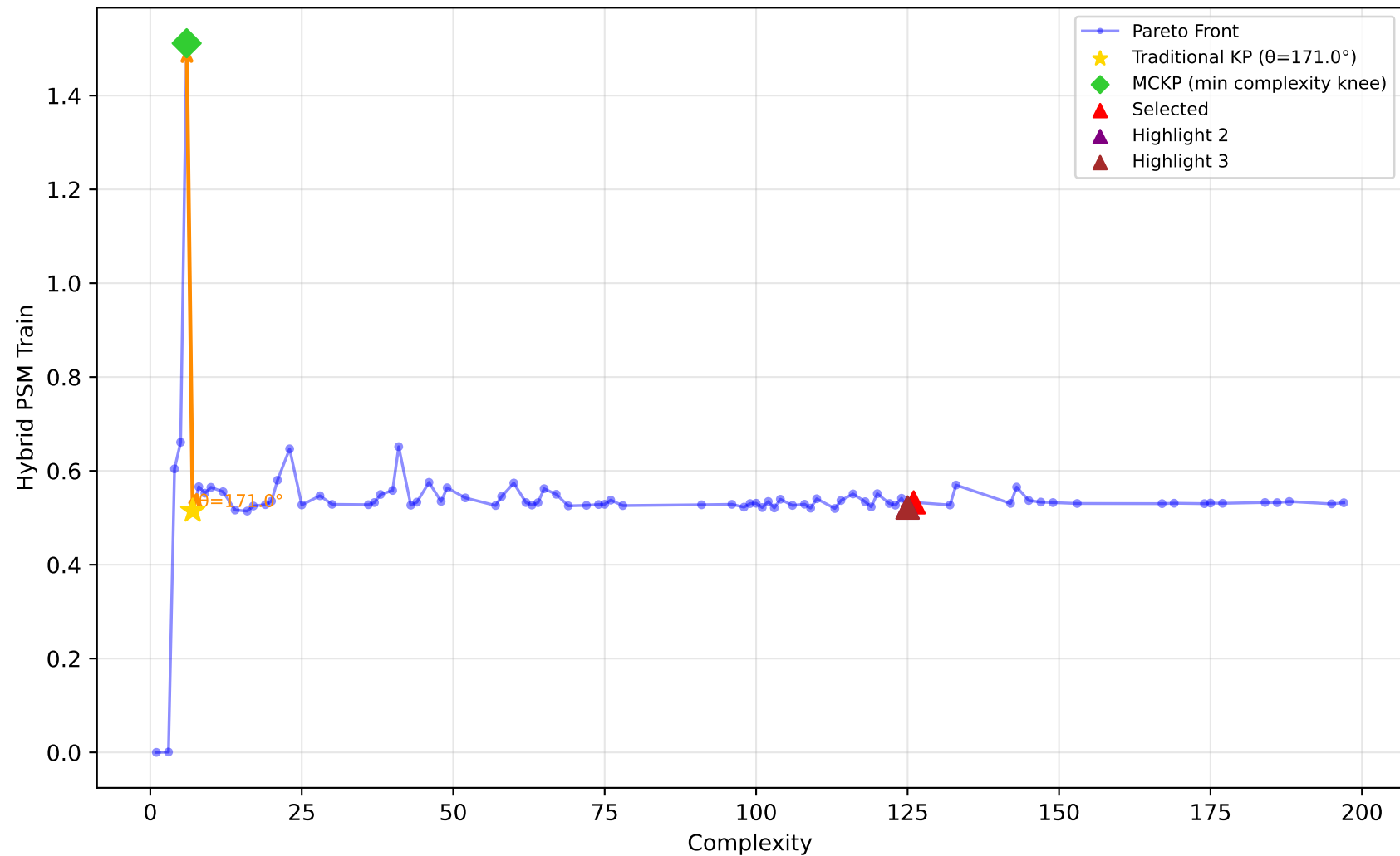
561_cpu - Run 2 - SVP - Hybrid PSM Train \lambda_1=1.00, \lambda_2=0.00, \lambda_3=0.40 | Difficulty: 0.51 | Method: mckp
