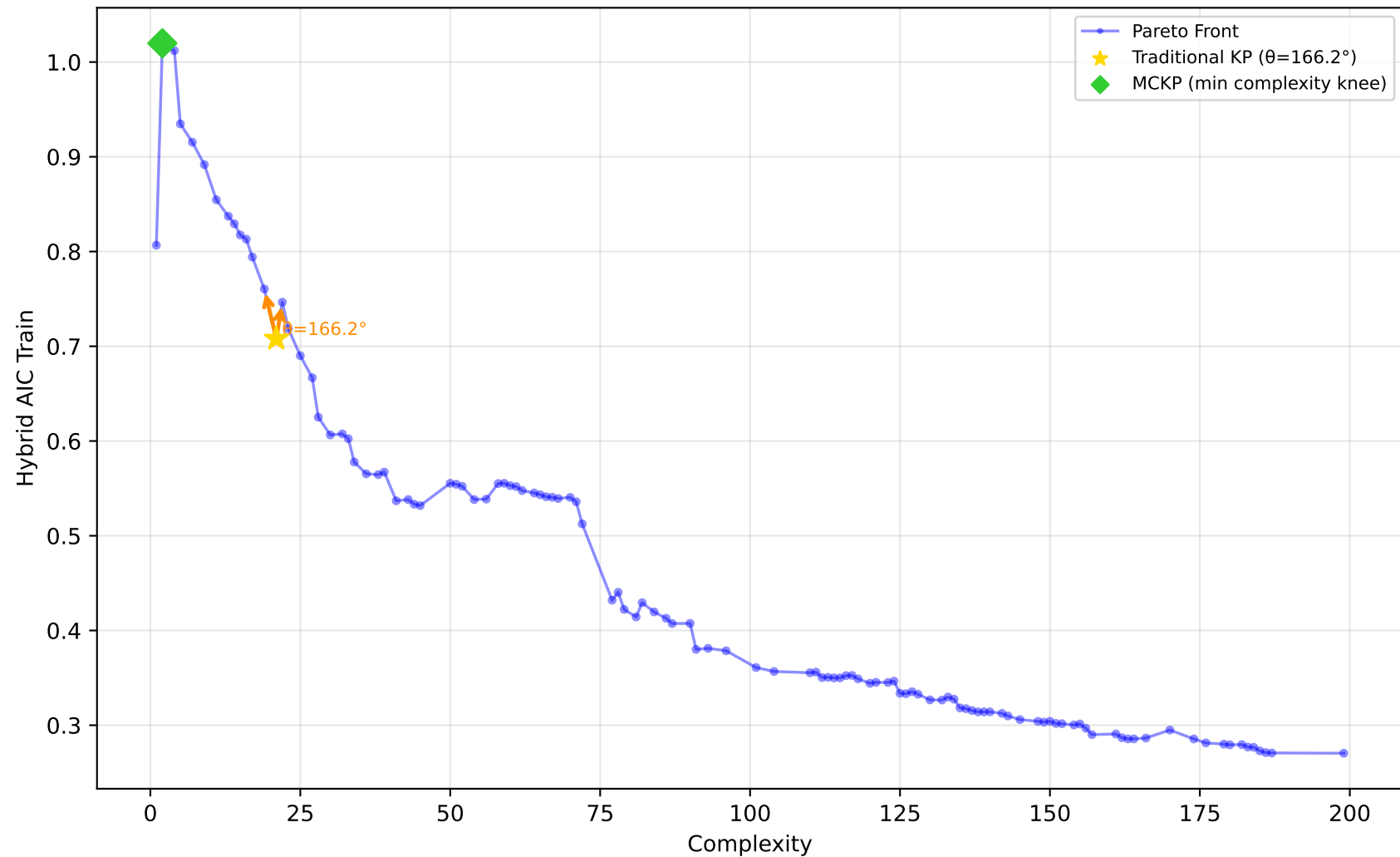
561_cpu - Run 30 - MVP - Hybrid AIC Train \lambda_1=0.50, \lambda_2=0.20, \lambda_3=0.00 | Difficulty: 1.00 | Method: hmr
