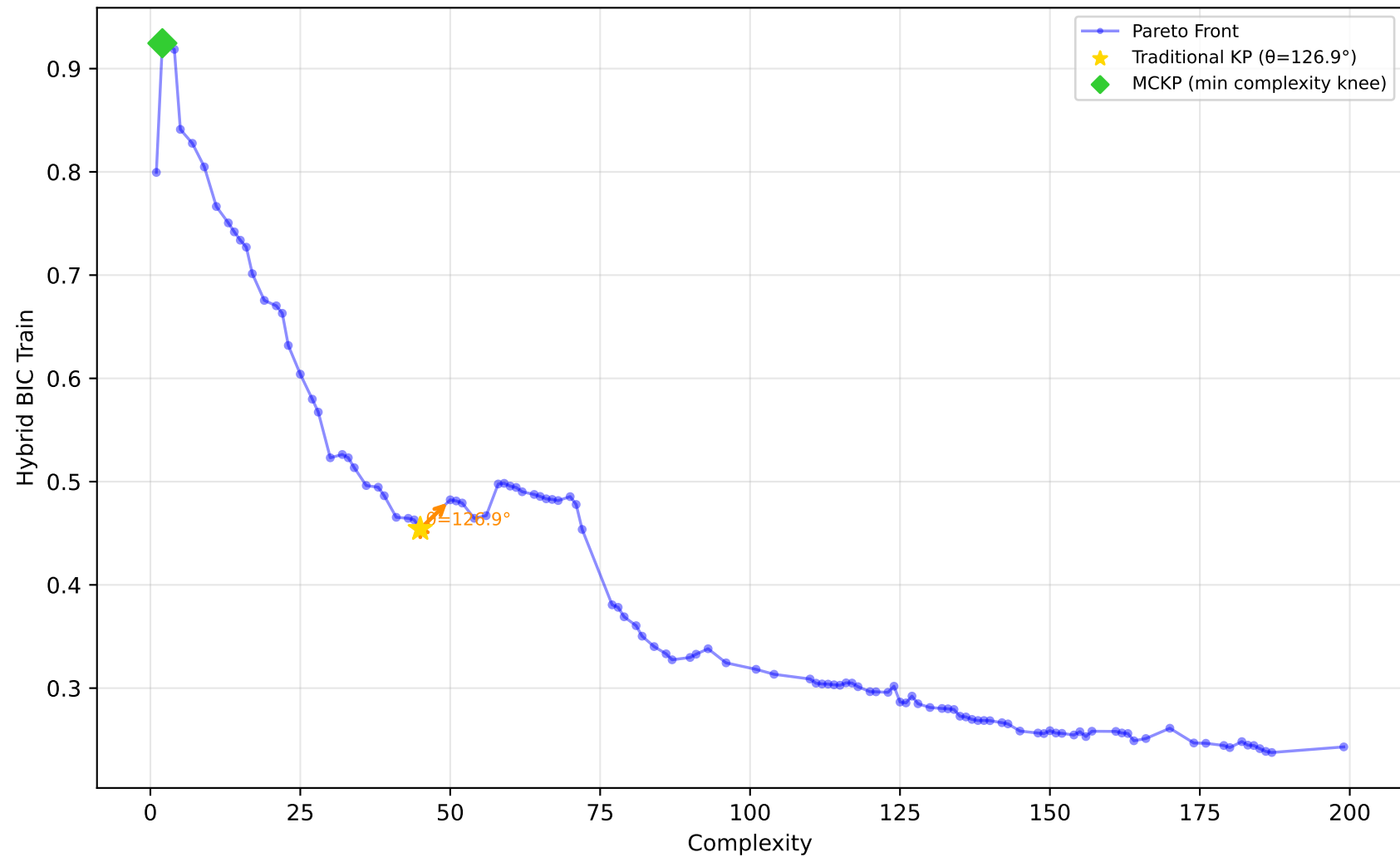
561_cpu - Run 30 - MVP - Hybrid BIC Train \lambda_1=0.70, \lambda_2=0.00, \lambda_3=0.10 | Difficulty: 1.00 | Method: hmr
