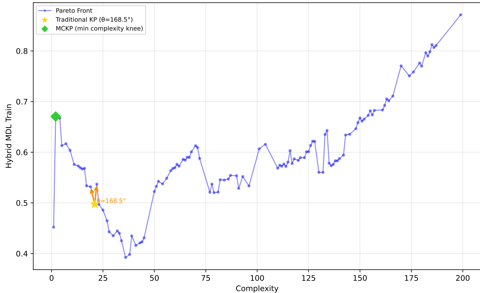
561_cpu - Run 30 - MVP - Hybrid MDL Train \lambda_1=0.50, \lambda_2=0.20, \lambda_3=0.00 | Difficulty: 1.00 | Method: hmr
