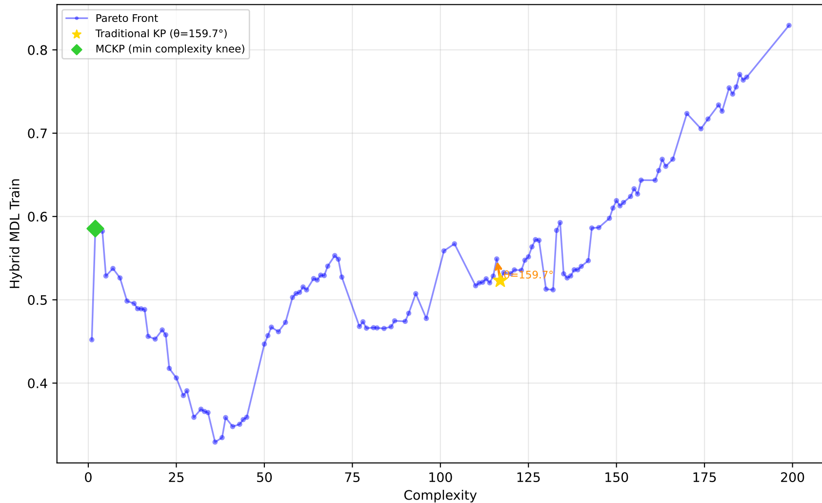
561_cpu - Run 30 - MVP - Hybrid MDL Train \lambda_1=0.70, \lambda_2=0.00, \lambda_3=0.10 | Difficulty: 1.00 | Method: hmr
