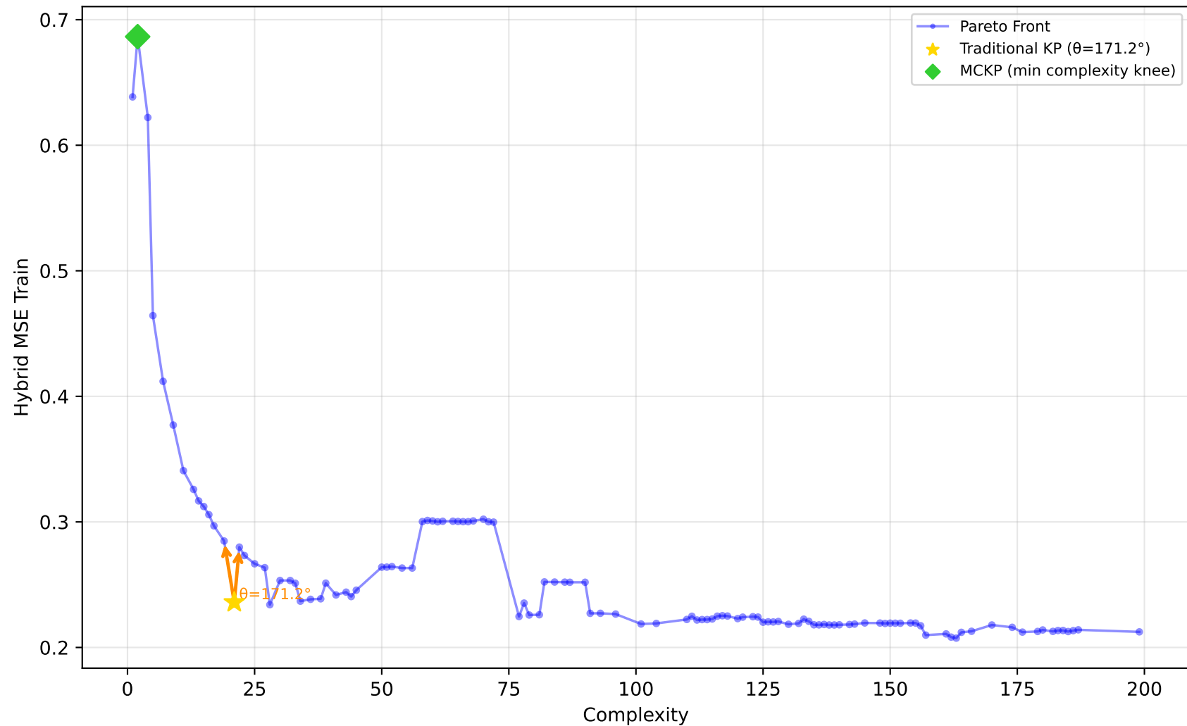
561_cpu - Run 30 - MVP - Hybrid MSE Train \lambda_1=0.50, \lambda_2=0.20, \lambda_3=0.00 | Difficulty: 1.00 | Method: hmr
