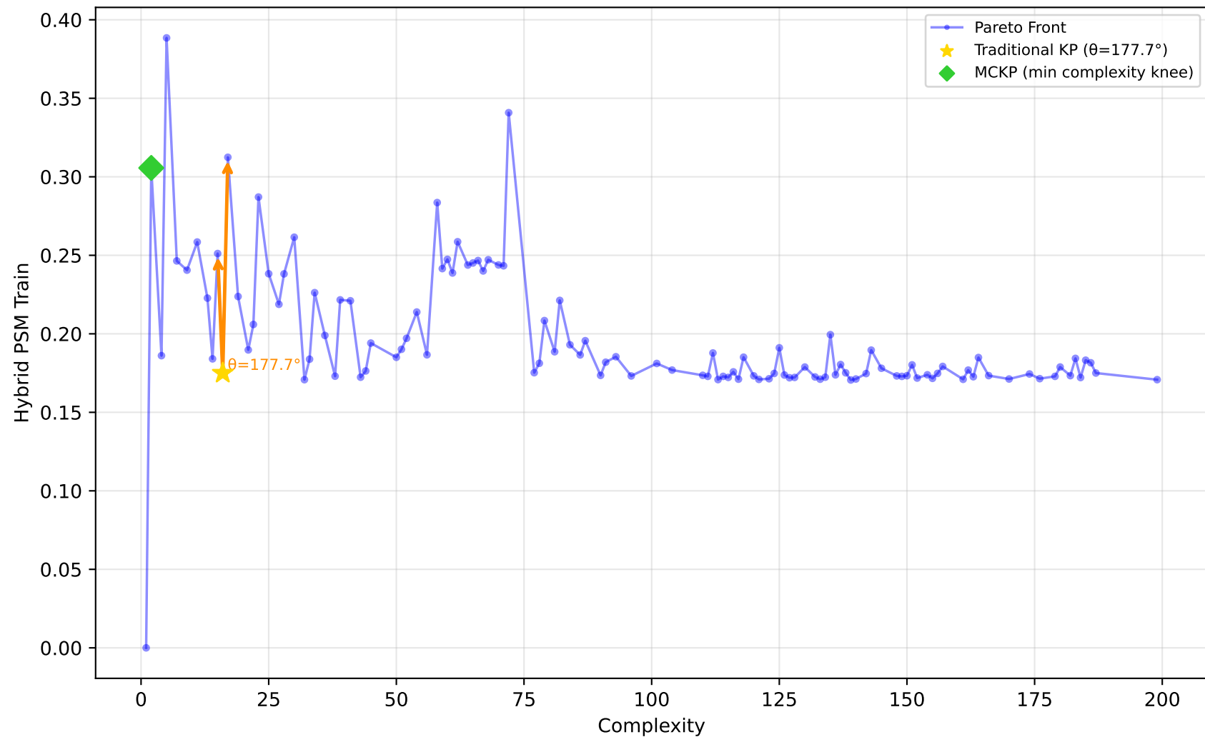
561_cpu - Run 30 - MVP - Hybrid PSM Train \lambda_1=0.70, \lambda_2=0.00, \lambda_3=0.10 | Difficulty: 1.00 | Method: hmr
