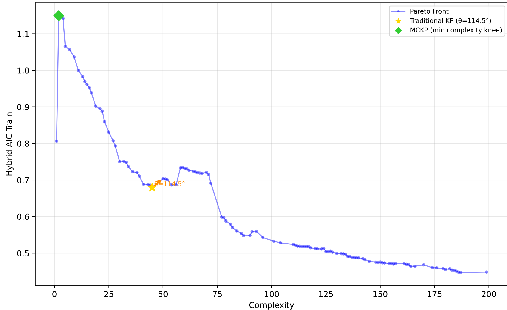
561_cpu - Run 30 - SVP - Hybrid AIC Train \lambda_1=0.90, \lambda_2=0.00, \lambda_3=0.30 | Difficulty: 1.00 | Method: hmr
