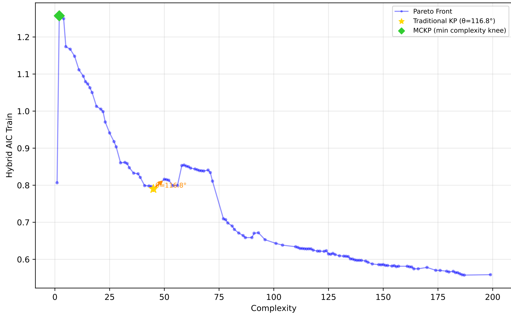
561_cpu - Run 30 - SVP - Hybrid AIC Train \lambda_1=1.00, \lambda_2=0.00, \lambda_3=0.40 | Difficulty: 1.00 | Method: hmr
