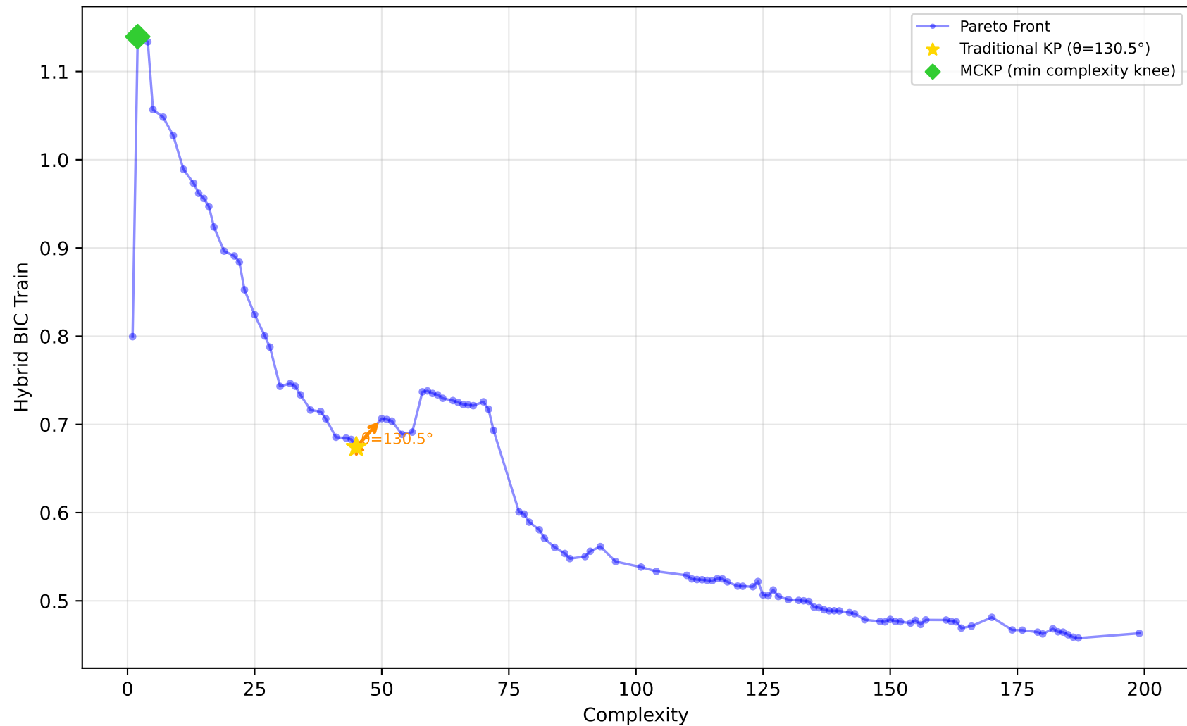
561_cpu - Run 30 - SVP - Hybrid BIC Train \lambda_1=0.90, \lambda_2=0.00, \lambda_3=0.30 | Difficulty: 1.00 | Method: hmr
