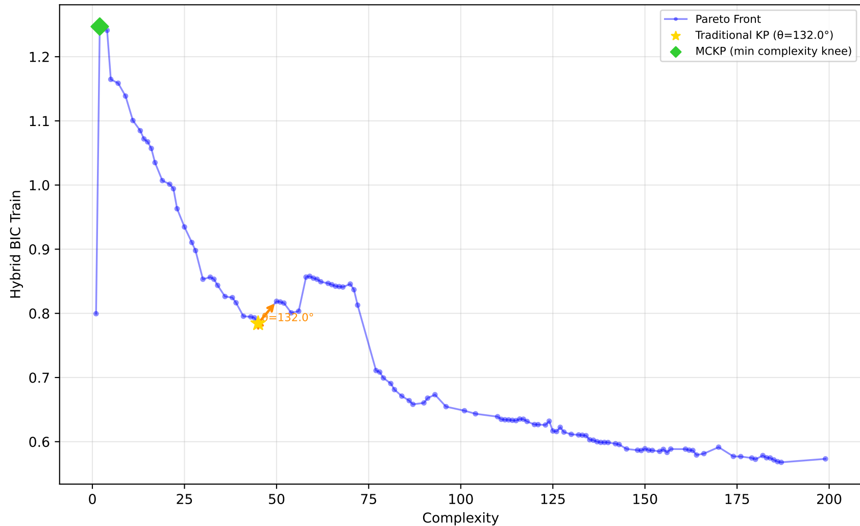
561_cpu - Run 30 - SVP - Hybrid BIC Train \lambda_1=1.00, \lambda_2=0.00, \lambda_3=0.40 | Difficulty: 1.00 | Method: hmr
