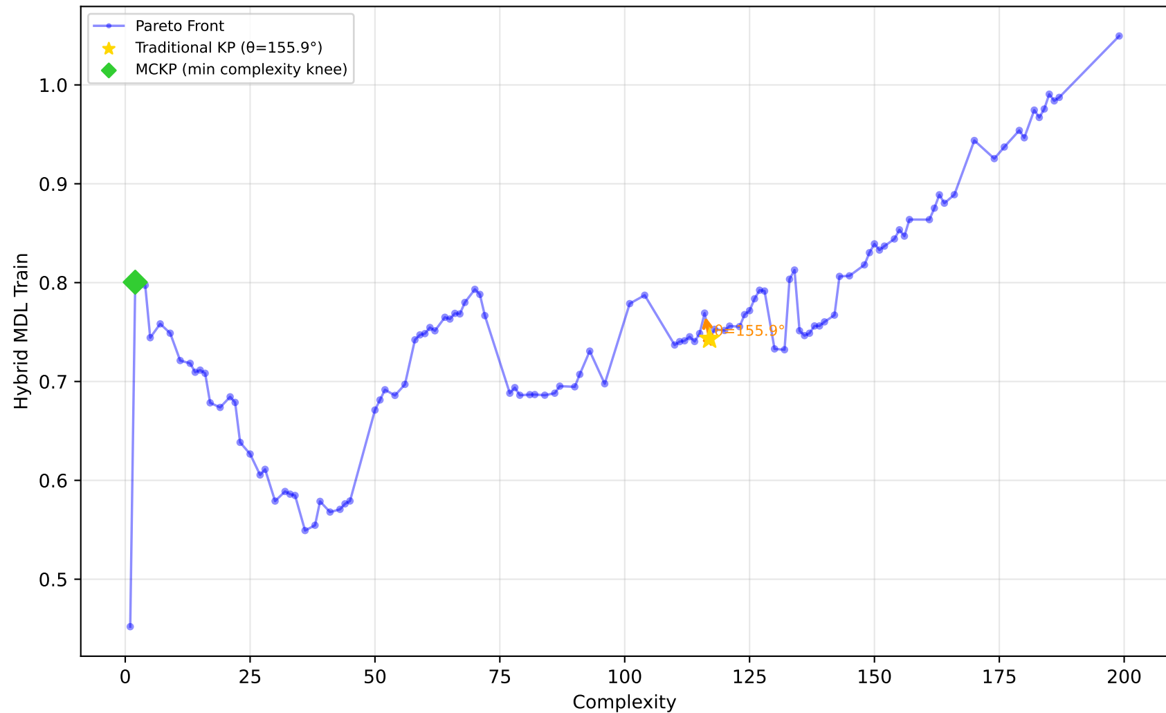
561_cpu - Run 30 - SVP - Hybrid MDL Train \lambda_1=0.90, \lambda_2=0.00, \lambda_3=0.30 | Difficulty: 1.00 | Method: hmr
