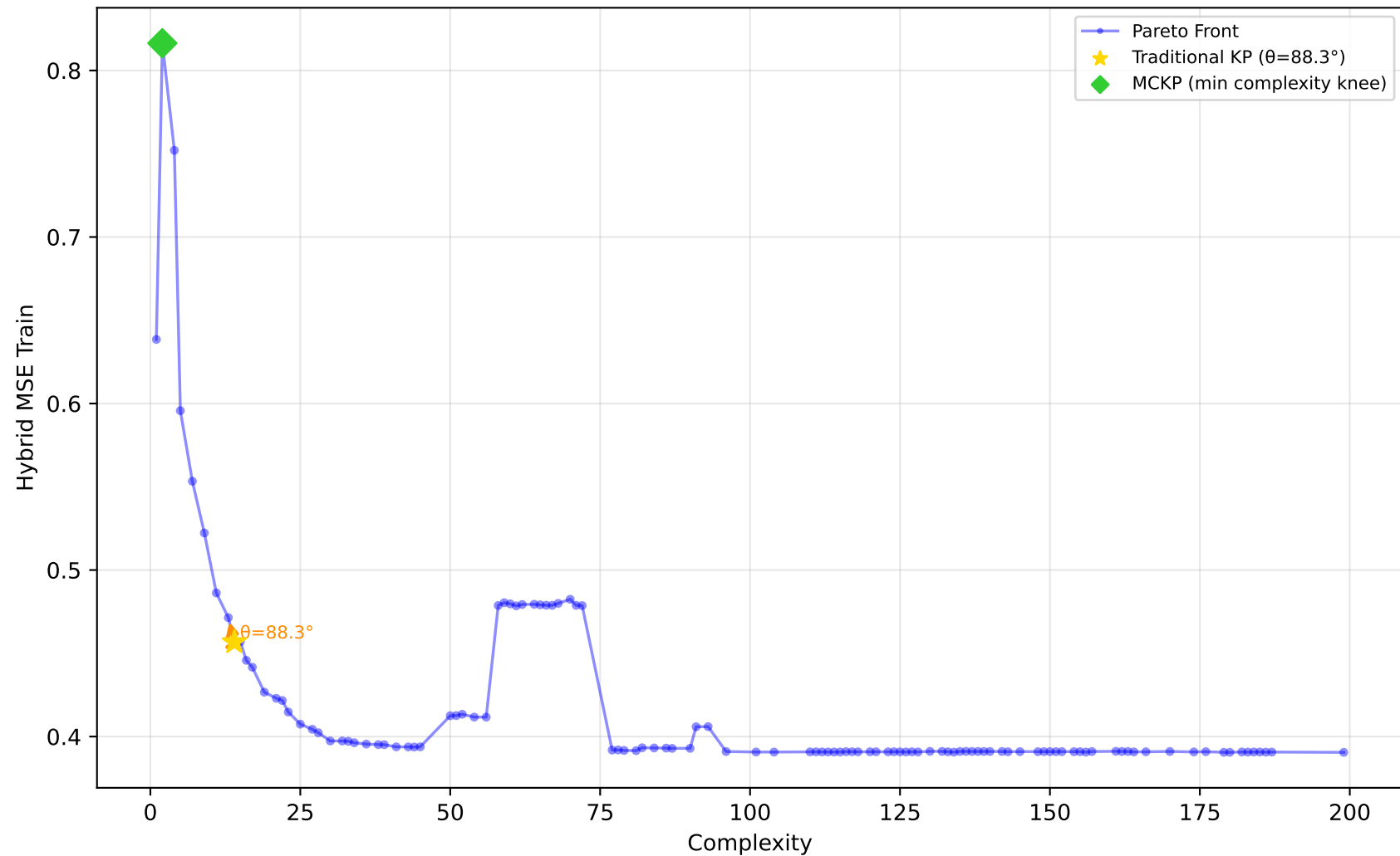
561_cpu - Run 30 - SVP - Hybrid MSE Train \lambda_1=0.90, \lambda_2=0.00, \lambda_3=0.30 | Difficulty: 1.00 | Method: hmr
