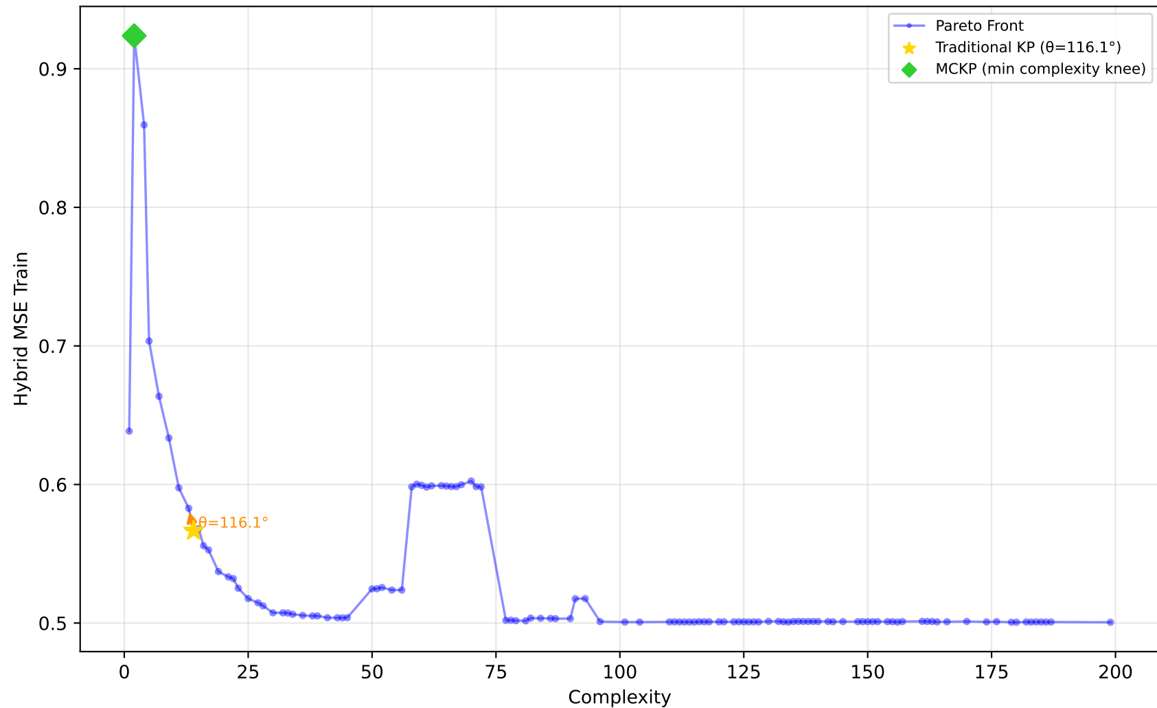
561_cpu - Run 30 - SVP - Hybrid MSE Train \lambda_1=1.00, \lambda_2=0.00, \lambda_3=0.40 | Difficulty: 1.00 | Method: hmr
