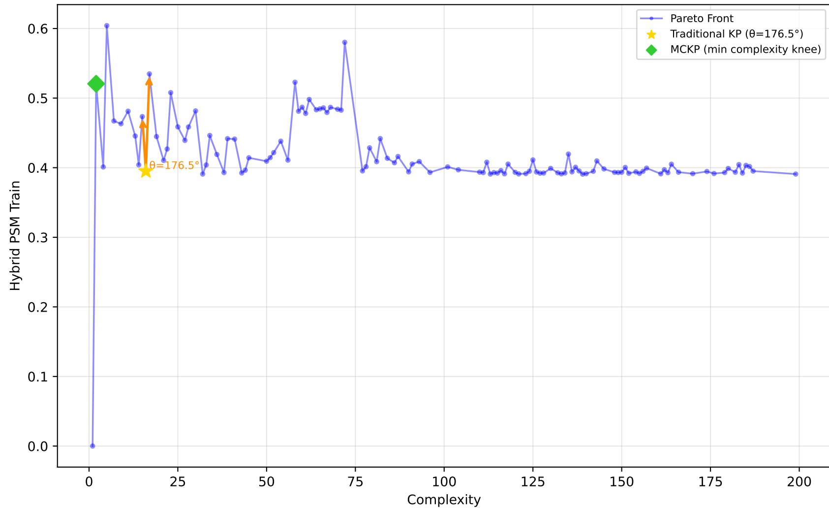
561_cpu - Run 30 - SVP - Hybrid PSM Train \lambda_1=0.90, \lambda_2=0.00, \lambda_3=0.30 | Difficulty: 1.00 | Method: hmr
