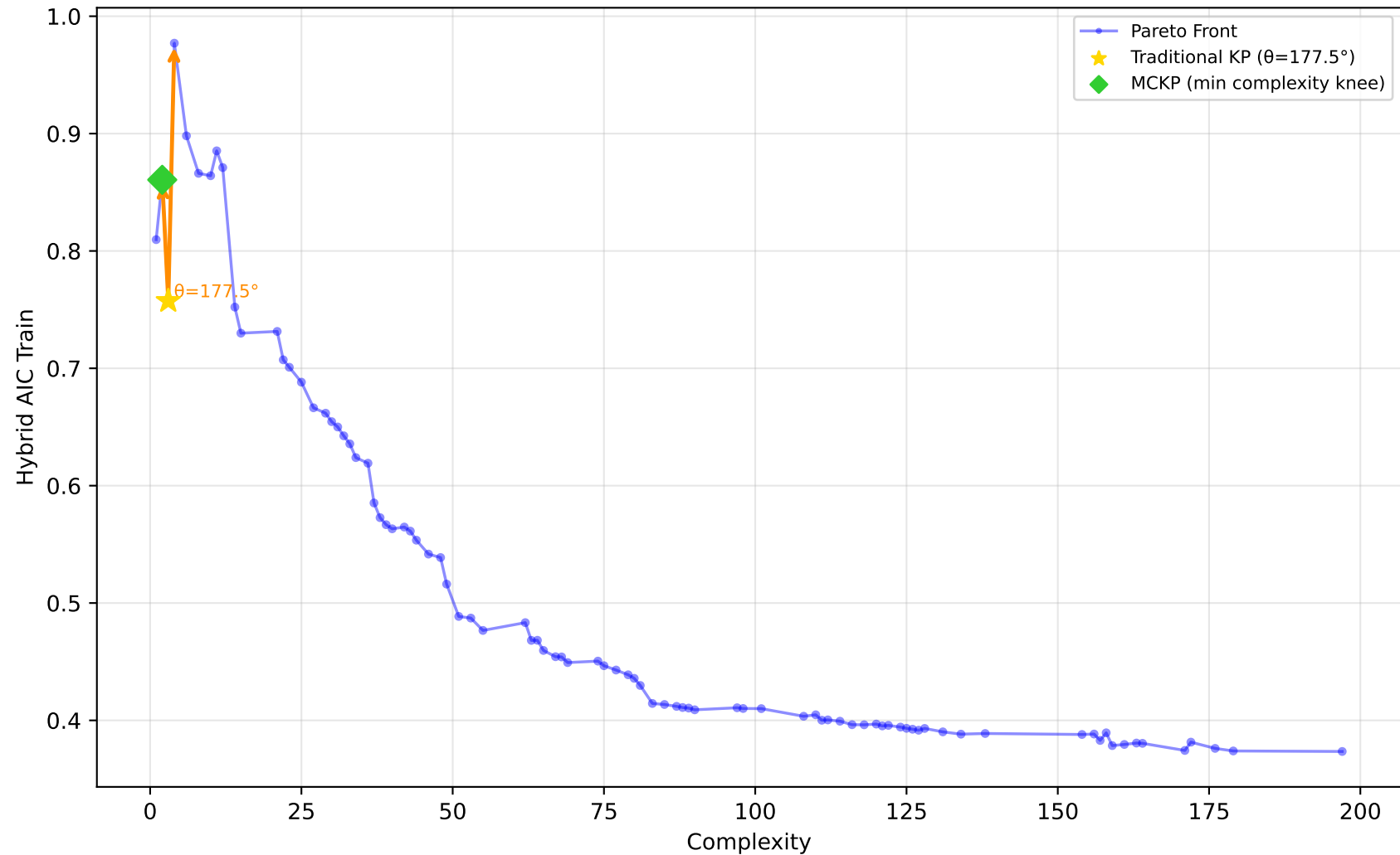
561_cpu - Run 3 - MVP - Hybrid AIC Train \lambda_1=0.50, \lambda_2=0.20, \lambda_3=0.00 | Difficulty: 1.00 | Method: hmr
