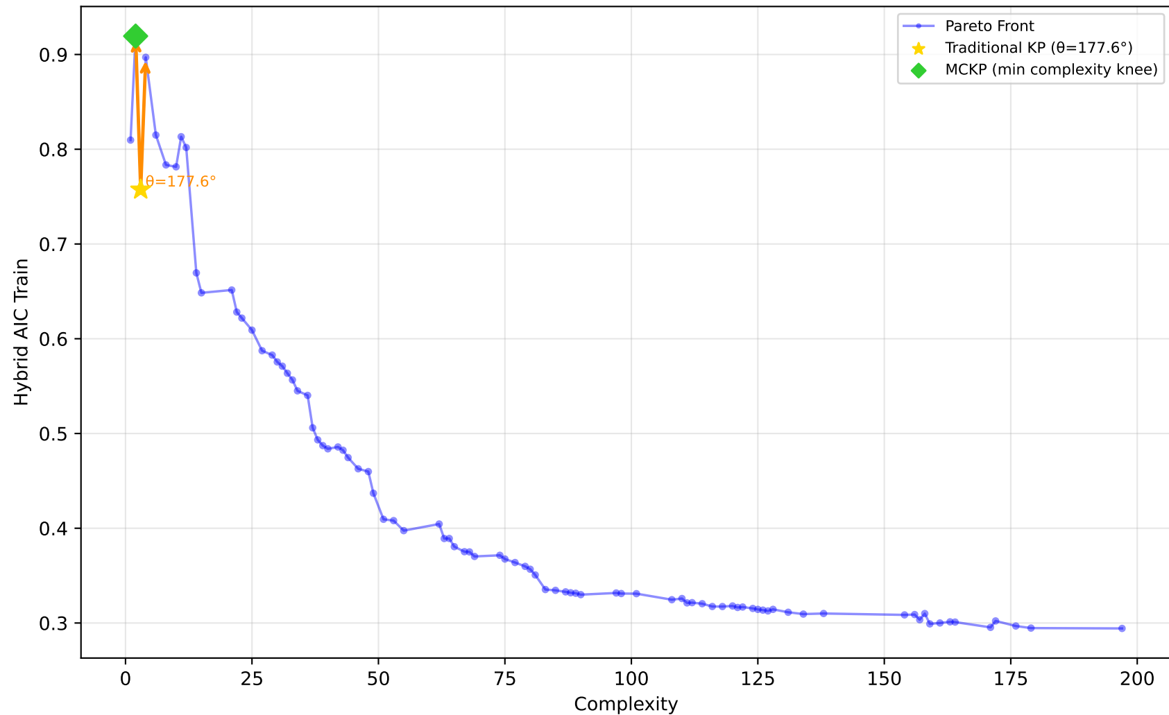
561_cpu - Run 3 - MVP - Hybrid AIC Train \lambda_1=0.70, \lambda_2=0.00, \lambda_3=0.10 | Difficulty: 1.00 | Method: hmr
