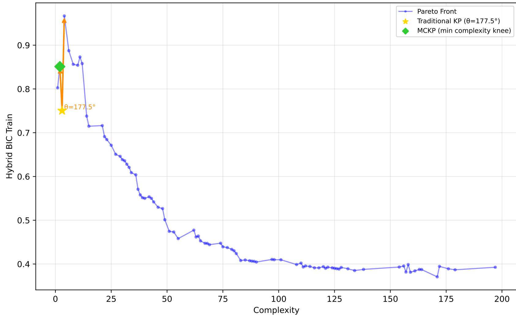
561_cpu - Run 3 - MVP - Hybrid BIC Train \lambda_1=0.50, \lambda_2=0.20, \lambda_3=0.00 | Difficulty: 1.00 | Method: hmr
