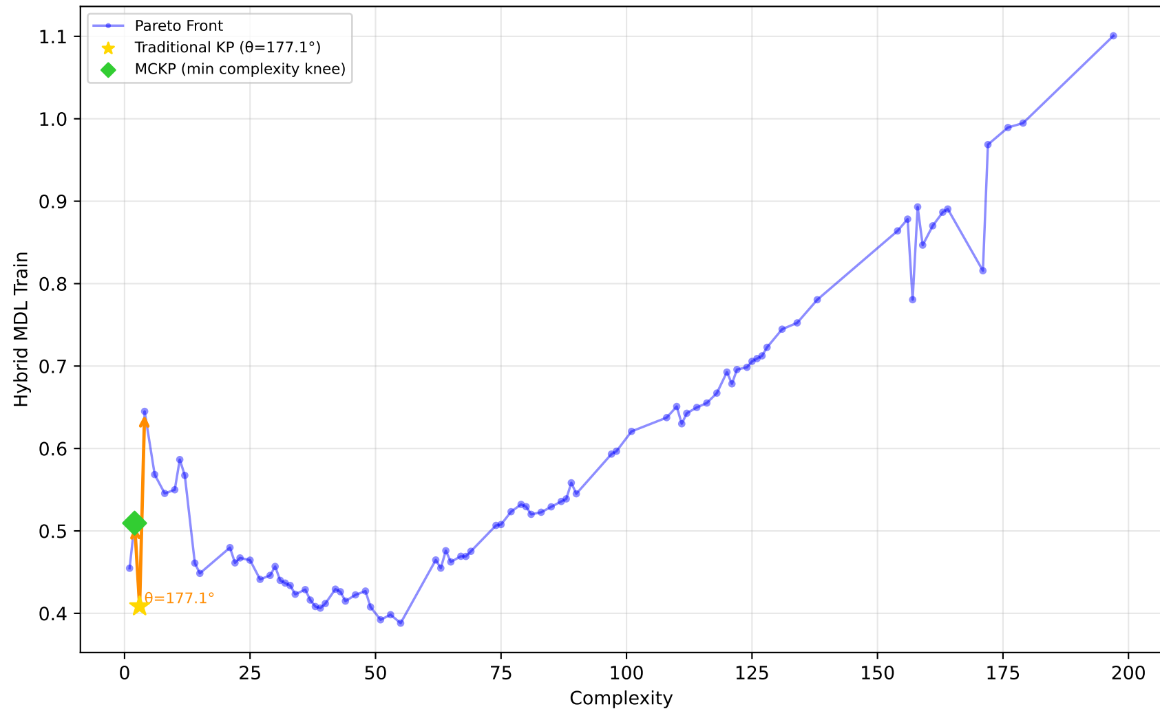
561_cpu - Run 3 - MVP - Hybrid MDL Train \lambda_1=0.50, \lambda_2=0.20, \lambda_3=0.00 | Difficulty: 1.00 | Method: hmr
