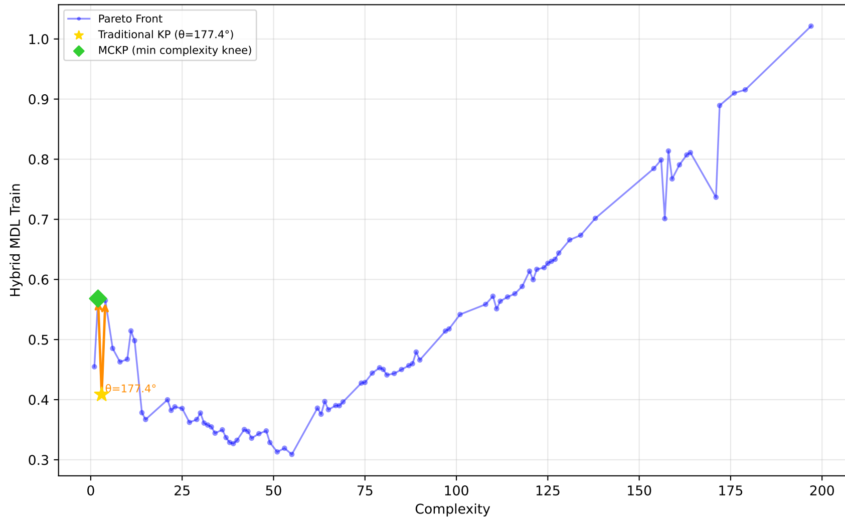
561_cpu - Run 3 - MVP - Hybrid MDL Train \lambda_1=0.70, \lambda_2=0.00, \lambda_3=0.10 | Difficulty: 1.00 | Method: hmr
