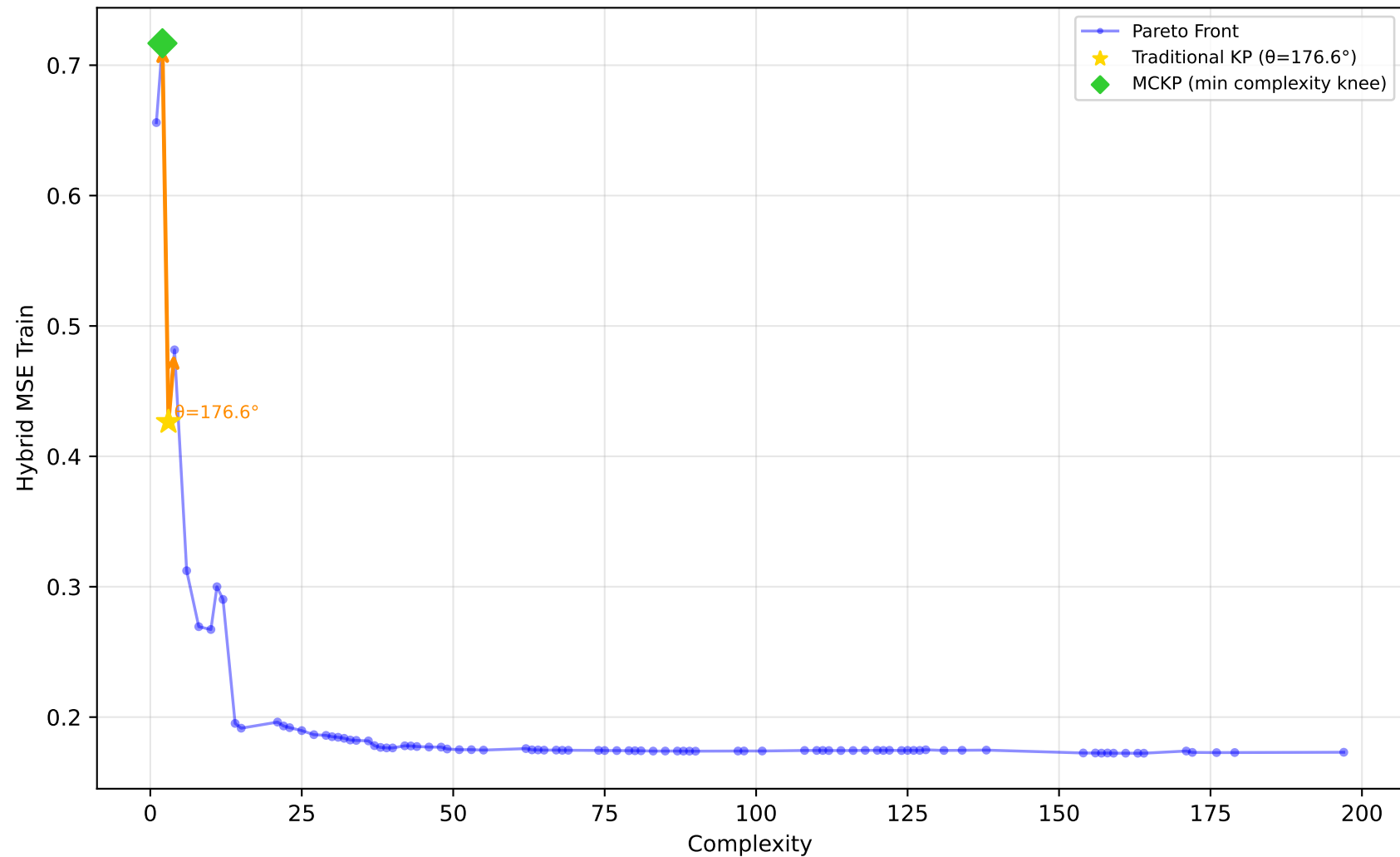
561_cpu - Run 3 - MVP - Hybrid MSE Train \lambda_1=0.70, \lambda_2=0.00, \lambda_3=0.10 | Difficulty: 1.00 | Method: hmr
