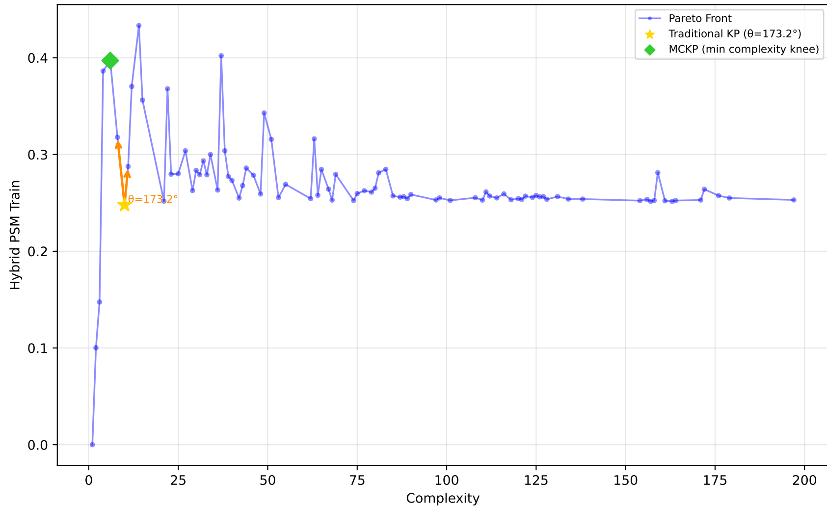
561_cpu - Run 3 - MVP - Hybrid PSM Train \lambda_1=0.50, \lambda_2=0.20, \lambda_3=0.00 | Difficulty: 1.00 | Method: hmr
