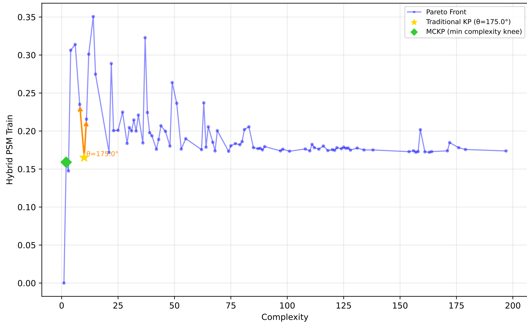
561_cpu - Run 3 - MVP - Hybrid PSM Train \lambda_1=0.70, \lambda_2=0.00, \lambda_3=0.10 | Difficulty: 1.00 | Method: hmr
