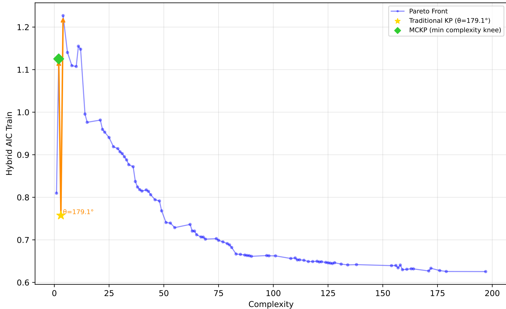
561_cpu - Run 3 - SVP - Hybrid AIC Train \lambda_1=1.00, \lambda_2=0.00, \lambda_3=0.40 | Difficulty: 1.00 | Method: hmr
