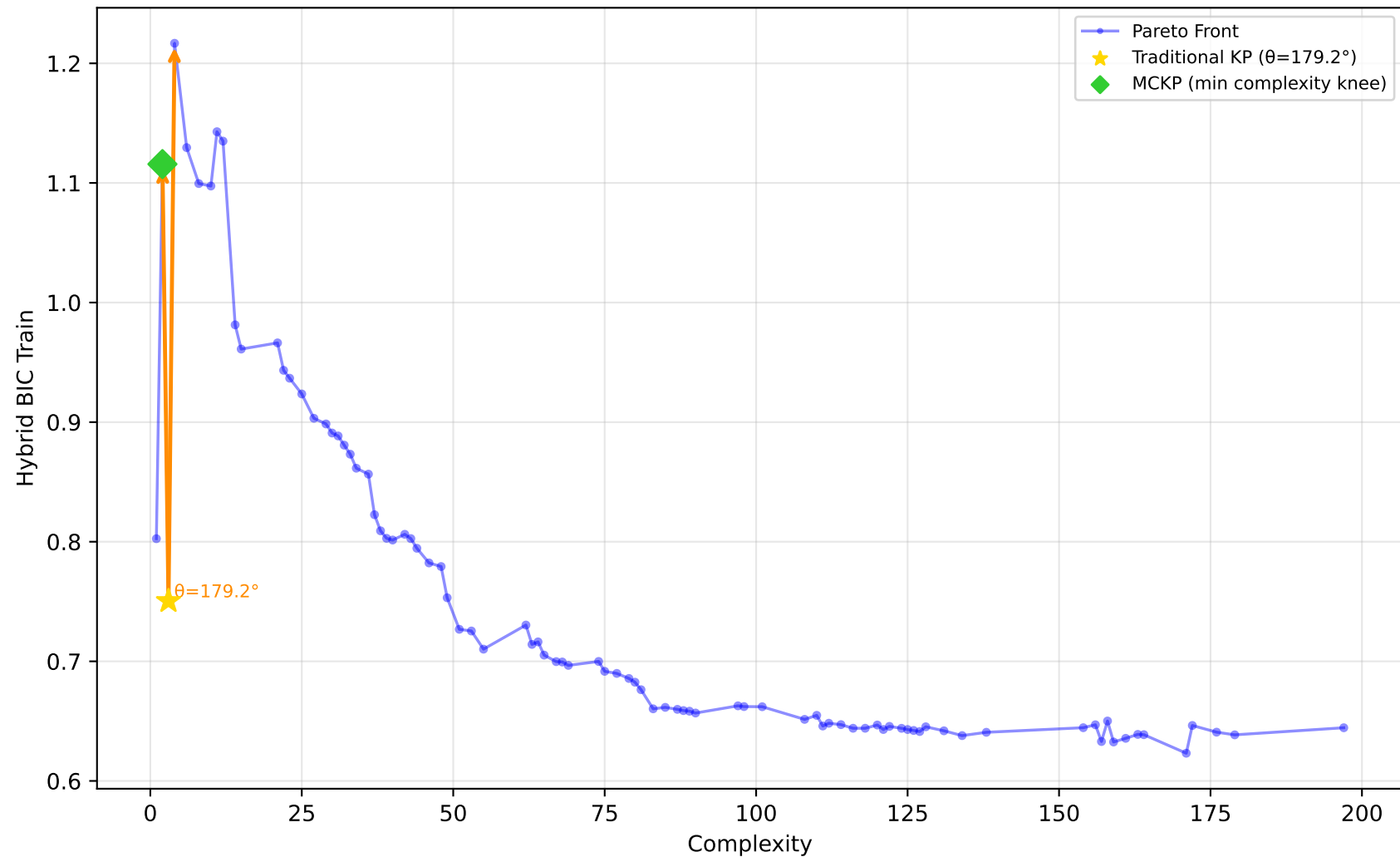
561_cpu - Run 3 - SVP - Hybrid BIC Train \lambda_1=1.00, \lambda_2=0.00, \lambda_3=0.40 | Difficulty: 1.00 | Method: hmr
