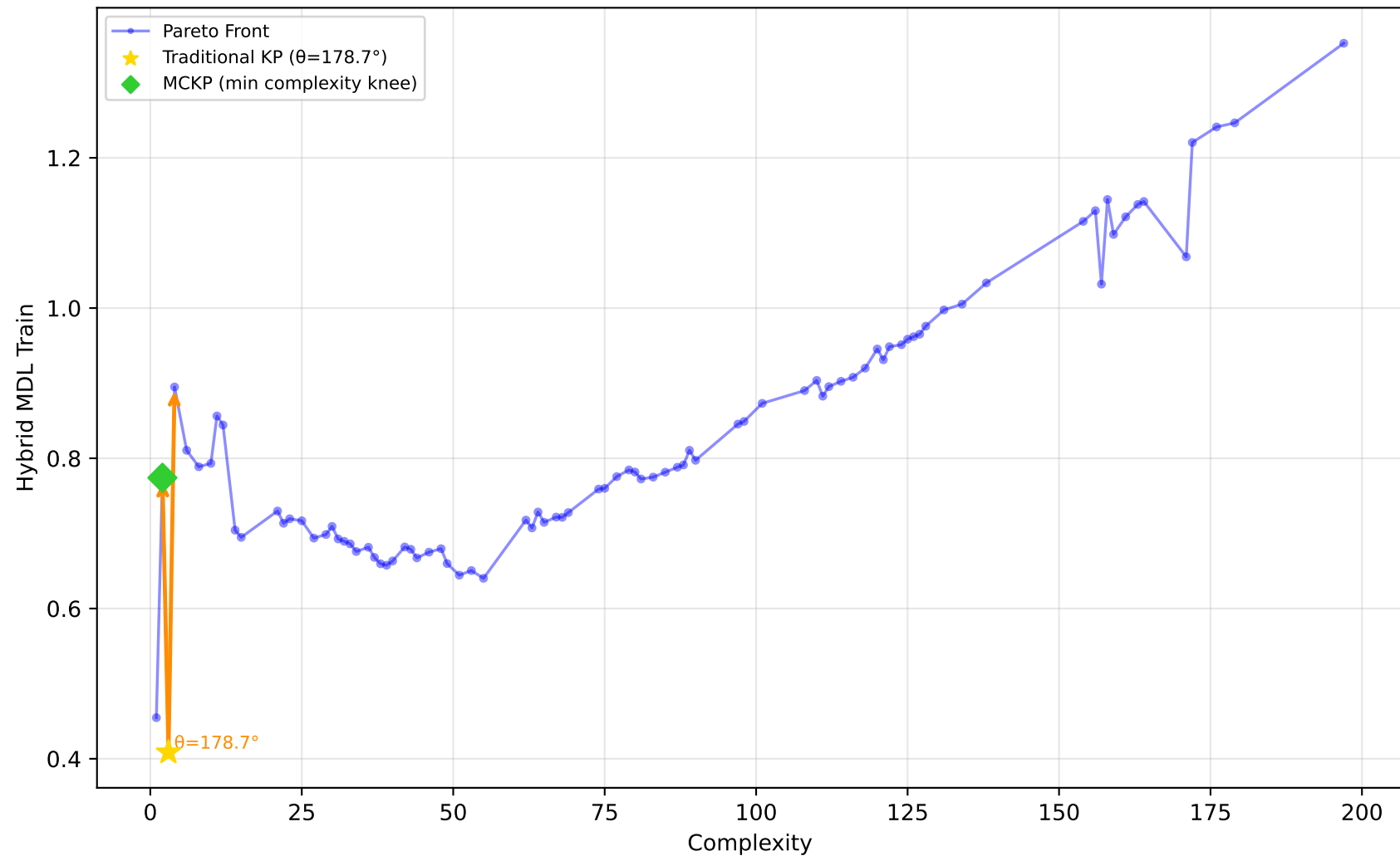
561_cpu - Run 3 - SVP - Hybrid MDL Train \lambda_1=1.00, \lambda_2=0.00, \lambda_3=0.40 | Difficulty: 1.00 | Method: hmr
