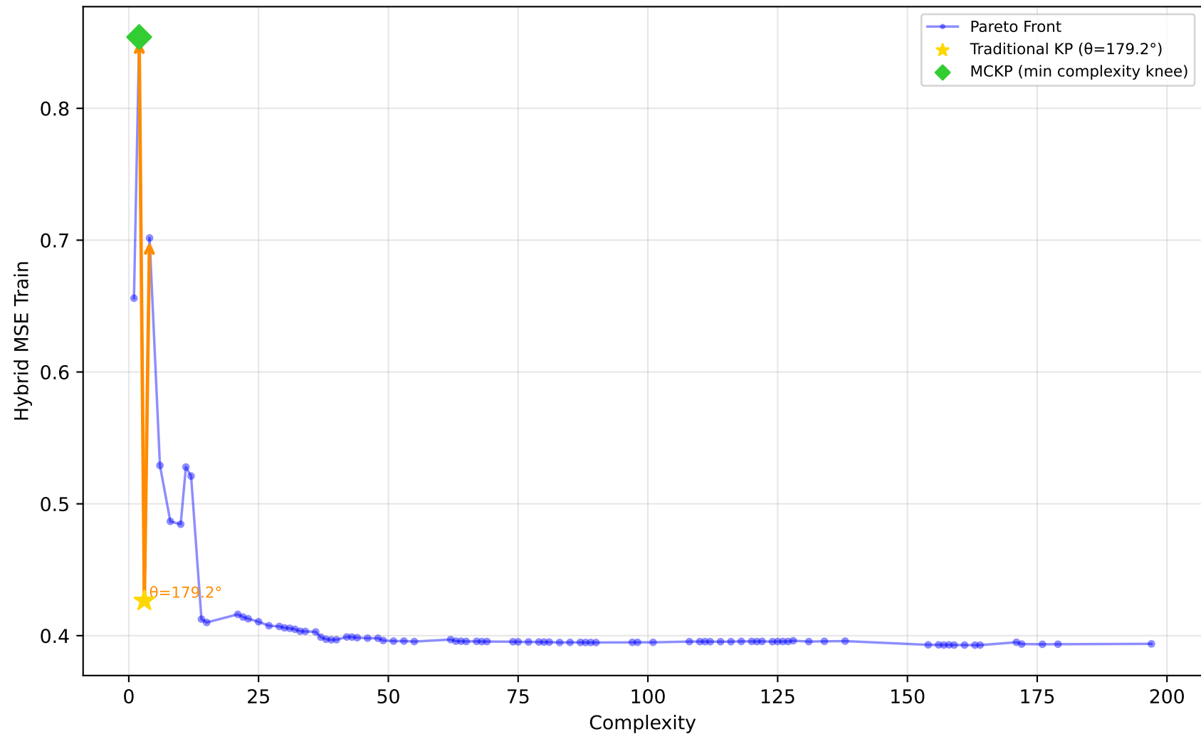
561_cpu - Run 3 - SVP - Hybrid MSE Train \lambda_1=0.90, \lambda_2=0.00, \lambda_3=0.30 | Difficulty: 1.00 | Method: hmr
