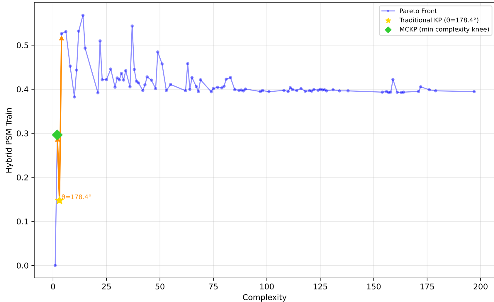
561_cpu - Run 3 - SVP - Hybrid PSM Train \lambda_1=0.90, \lambda_2=0.00, \lambda_3=0.30 | Difficulty: 1.00 | Method: hmr
